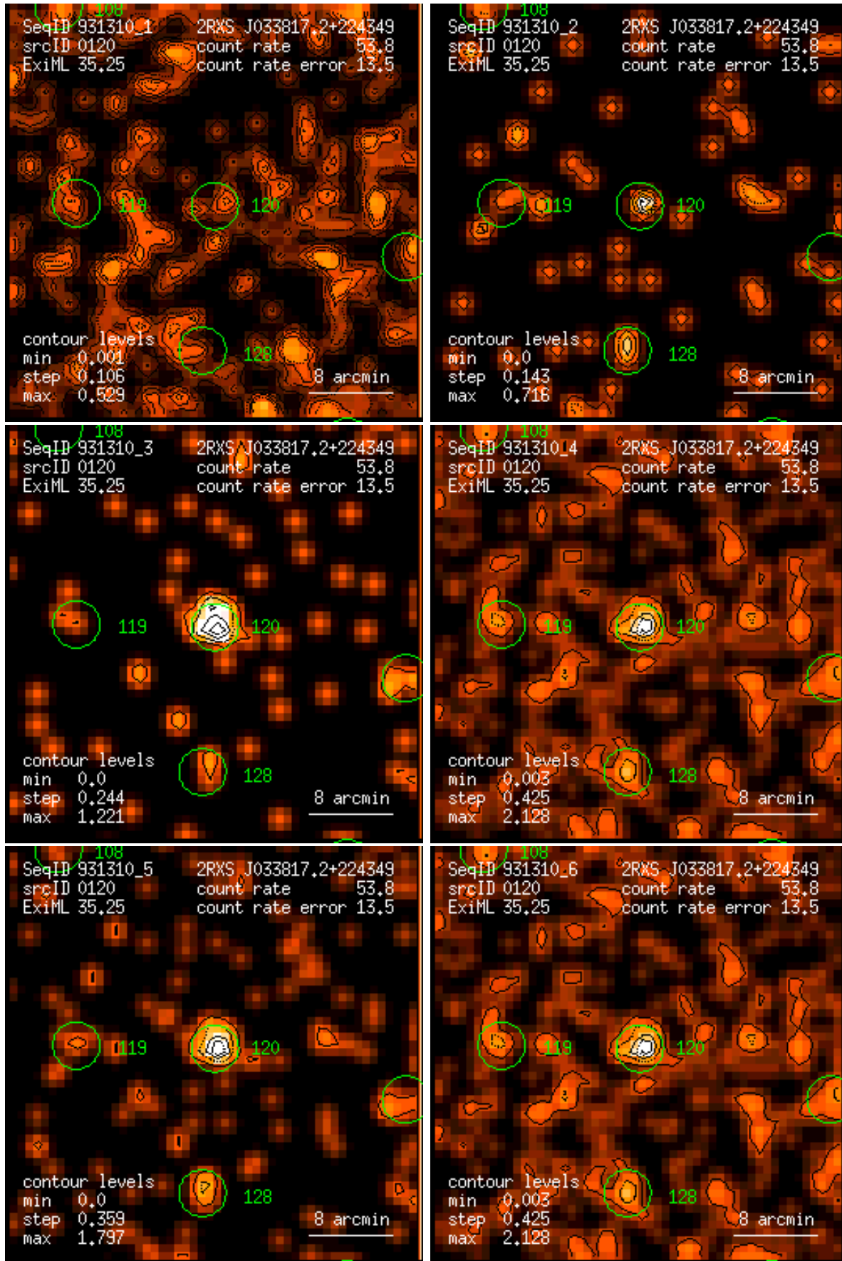
Figure 120: RASS 931310: detection 0120: band rate images, Gaussian filter: (1) PSPC channels 11 – 41, (2) 52 – 90, (3) 91 – 201, (4) 11 – 235, (5) 52 – 201, (6) 11 – 201. Broad band rates in counts/ks. Band rate contour levels in counts/ks/arcmin 2 .
