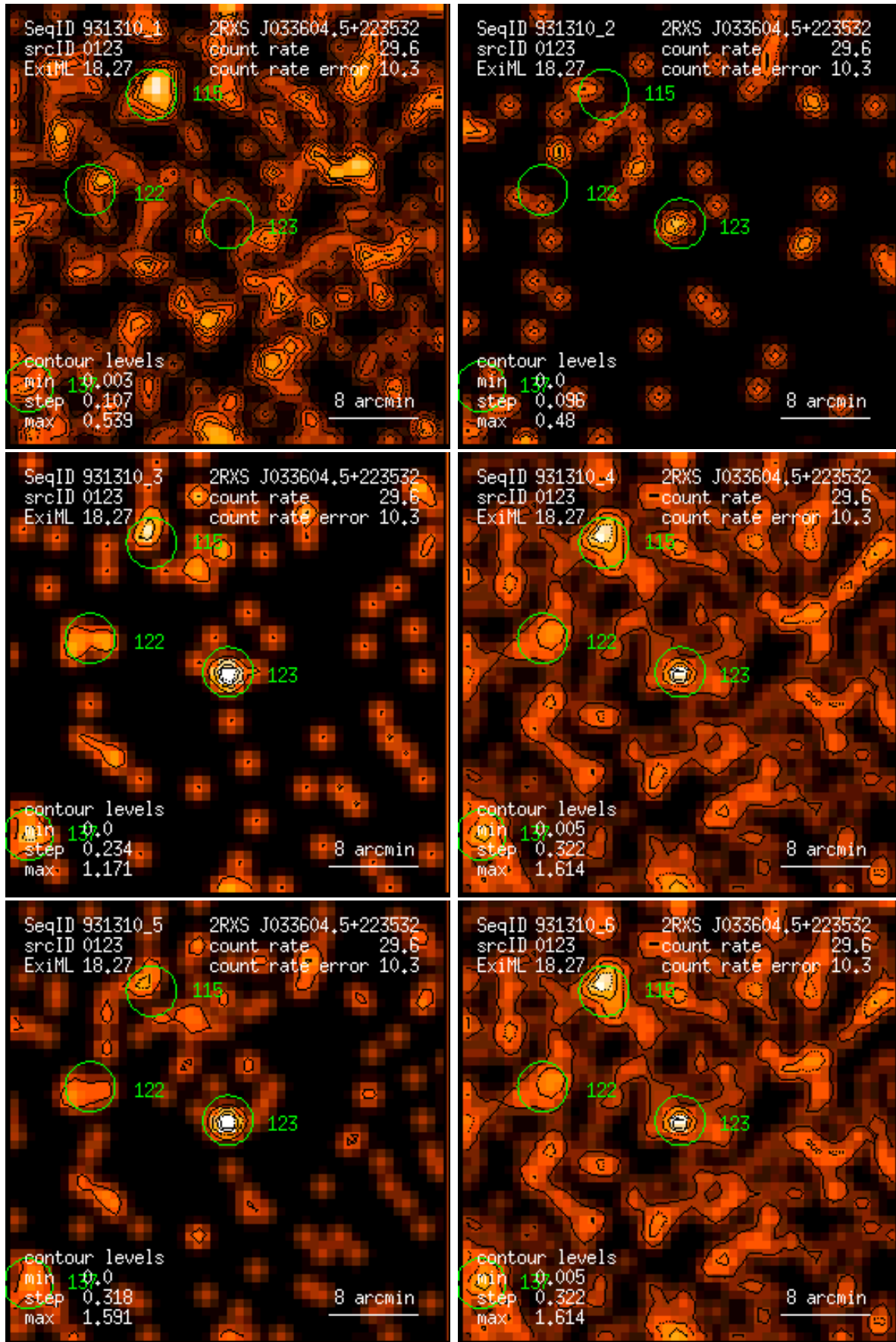
Figure 123: RASS 931310: detection 0123: band rate images, Gaussian filter: (1) PSPC channels 11 – 41, (2) 52 – 90, (3) 91 – 201, (4) 11 – 235, (5) 52 – 201, (6) 11 – 201. Broad band rates in counts/ks. Band rate contour levels in counts/ks/arcmin 2 .
