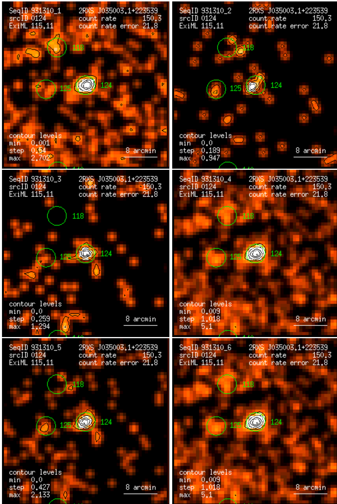
Figure 124: RASS 931310: detection 0124: band rate images, Gaussian filter: (1) PSPC channels 11 – 41, (2) 52 – 90, (3) 91 – 201, (4) 11 – 235, (5) 52 – 201, (6) 11 – 201. Broad band rates in counts/ks. Band rate contour levels in counts/ks/arcmin 2 .
