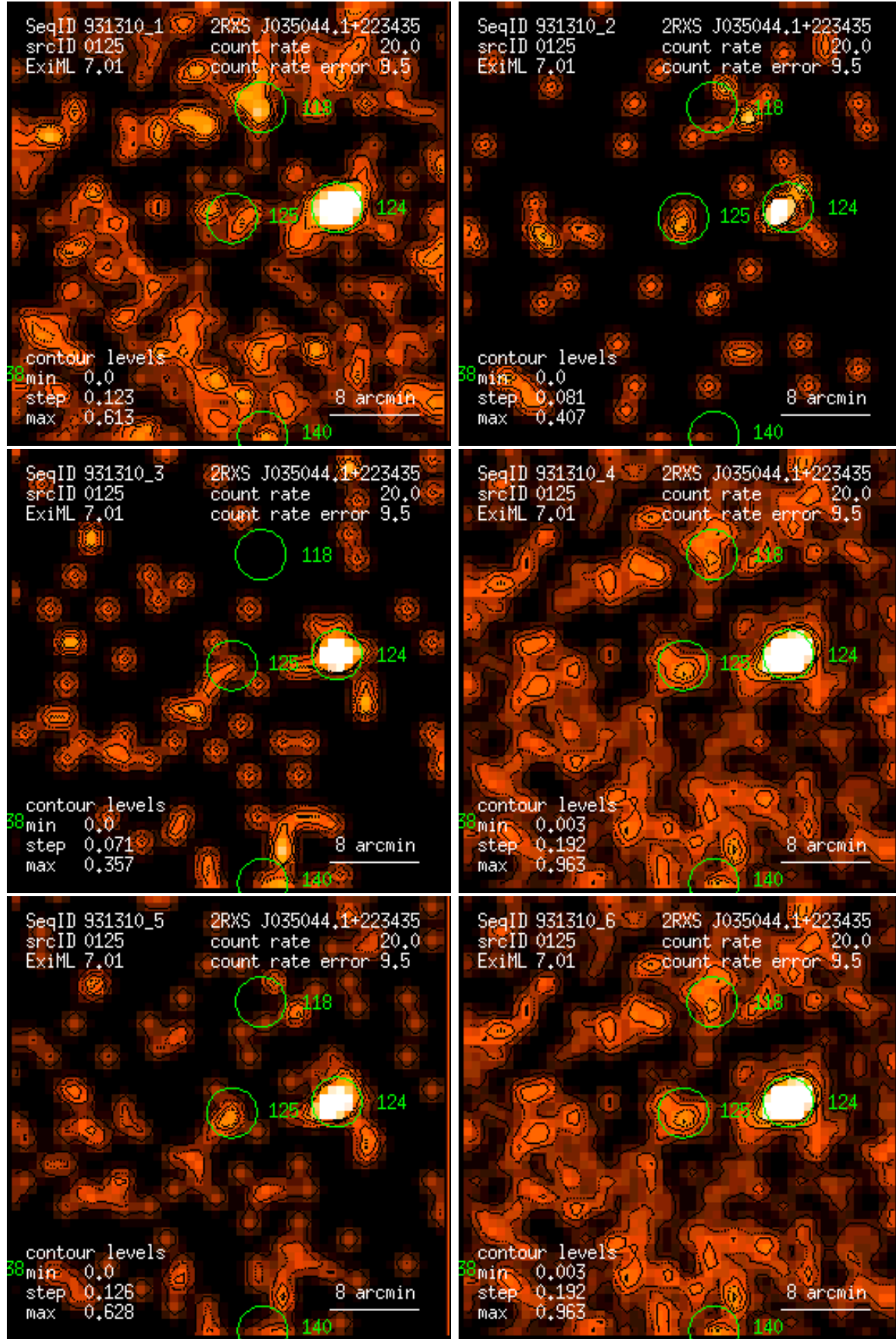
Figure 125: RASS 931310: detection 0125: band rate images, Gaussian filter: (1) PSPC channels 11 – 41, (2) 52 – 90, (3) 91 – 201, (4) 11 – 235, (5) 52 – 201, (6) 11 – 201. Broad band rates in counts/ks. Band rate contour levels in counts/ks/arcmin 2 .
