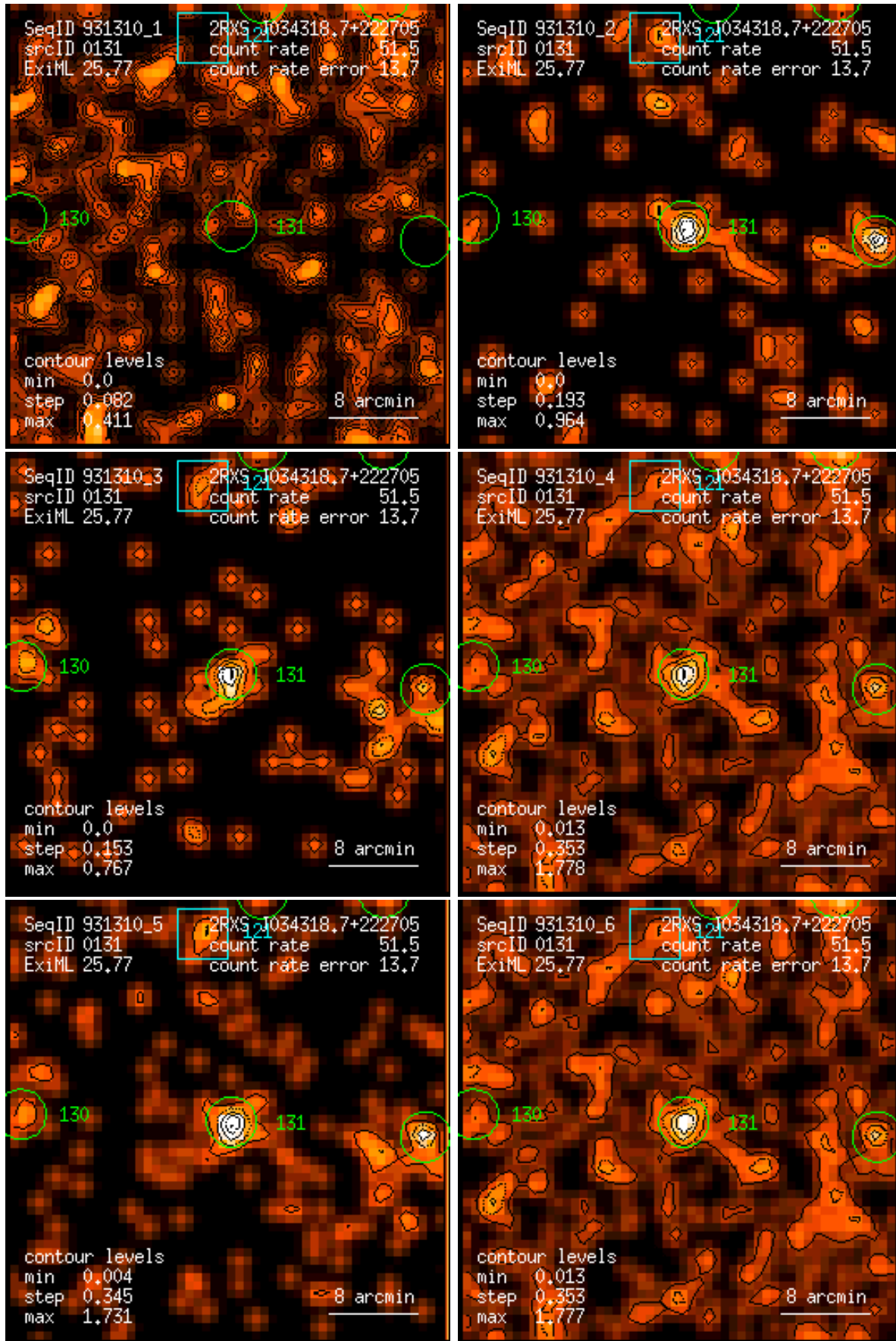
Figure 131: RASS 931310: detection 0131: band rate images, Gaussian filter: (1) PSPC channels 11 – 41, (2) 52 – 90, (3) 91 – 201, (4) 11 – 235, (5) 52 – 201, (6) 11 – 201. Broad band rates in counts/ks. Band rate contour levels in counts/ks/arcmin 2 .
