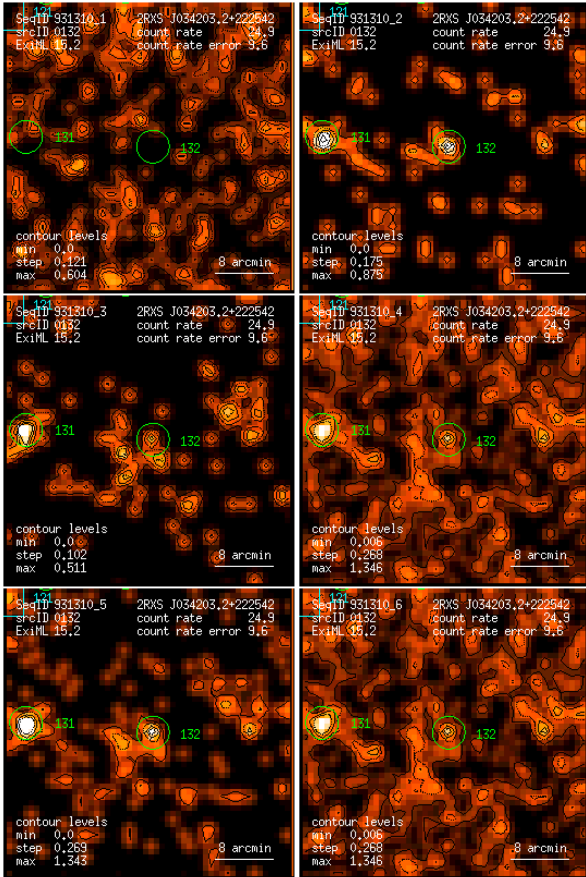
Figure 132: RASS 931310: detection 0132: band rate images, Gaussian filter: (1) PSPC channels 11 – 41, (2) 52 – 90, (3) 91 – 201, (4) 11 – 235, (5) 52 – 201, (6) 11 – 201. Broad band rates in counts/ks. Band rate contour levels in counts/ks/arcmin 2 .
