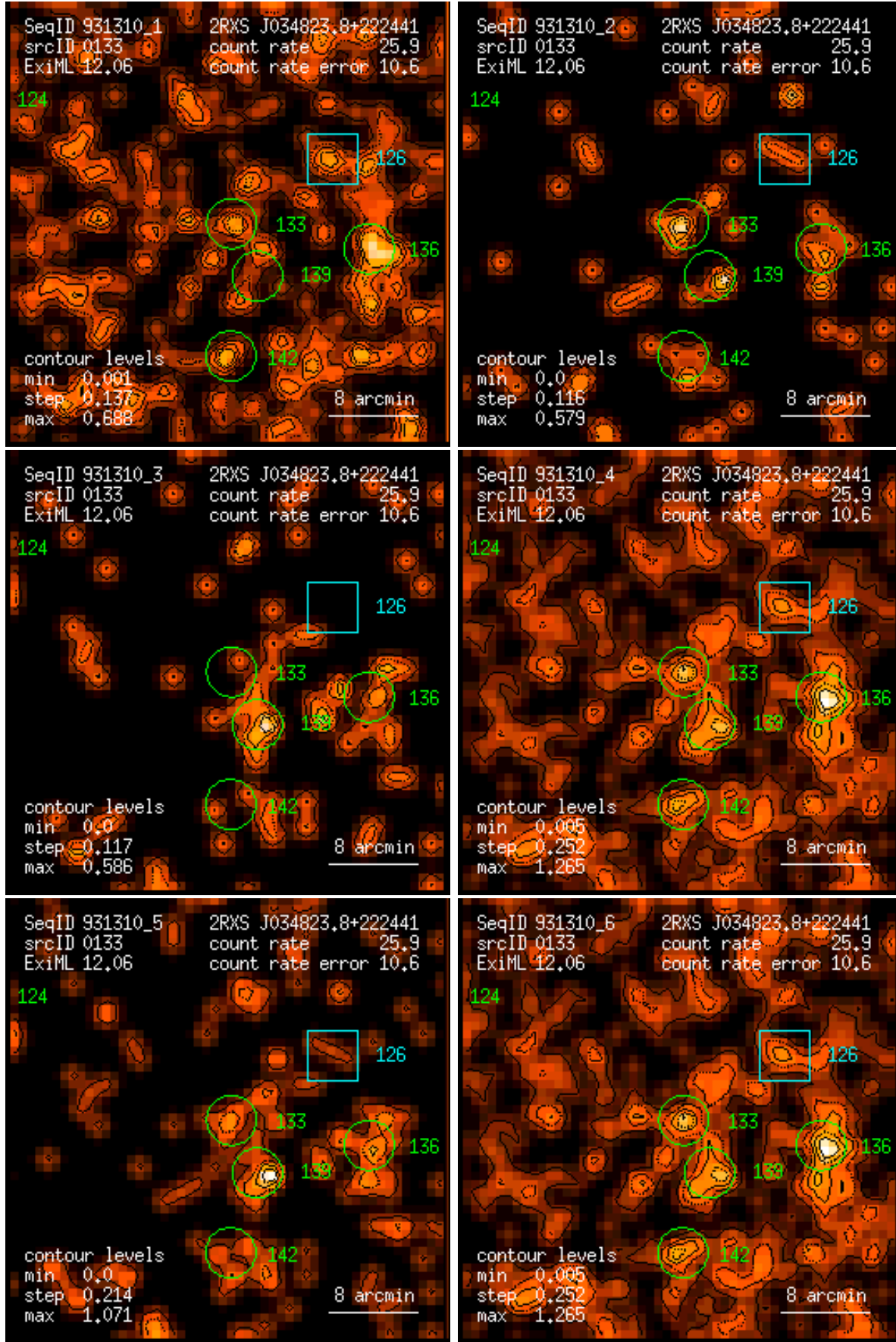
Figure 133: RASS 931310: detection 0133: band rate images, Gaussian filter: (1) PSPC channels 11 – 41, (2) 52 – 90, (3) 91 – 201, (4) 11 – 235, (5) 52 – 201, (6) 11 – 201. Broad band rates in counts/ks. Band rate contour levels in counts/ks/arcmin 2 .
