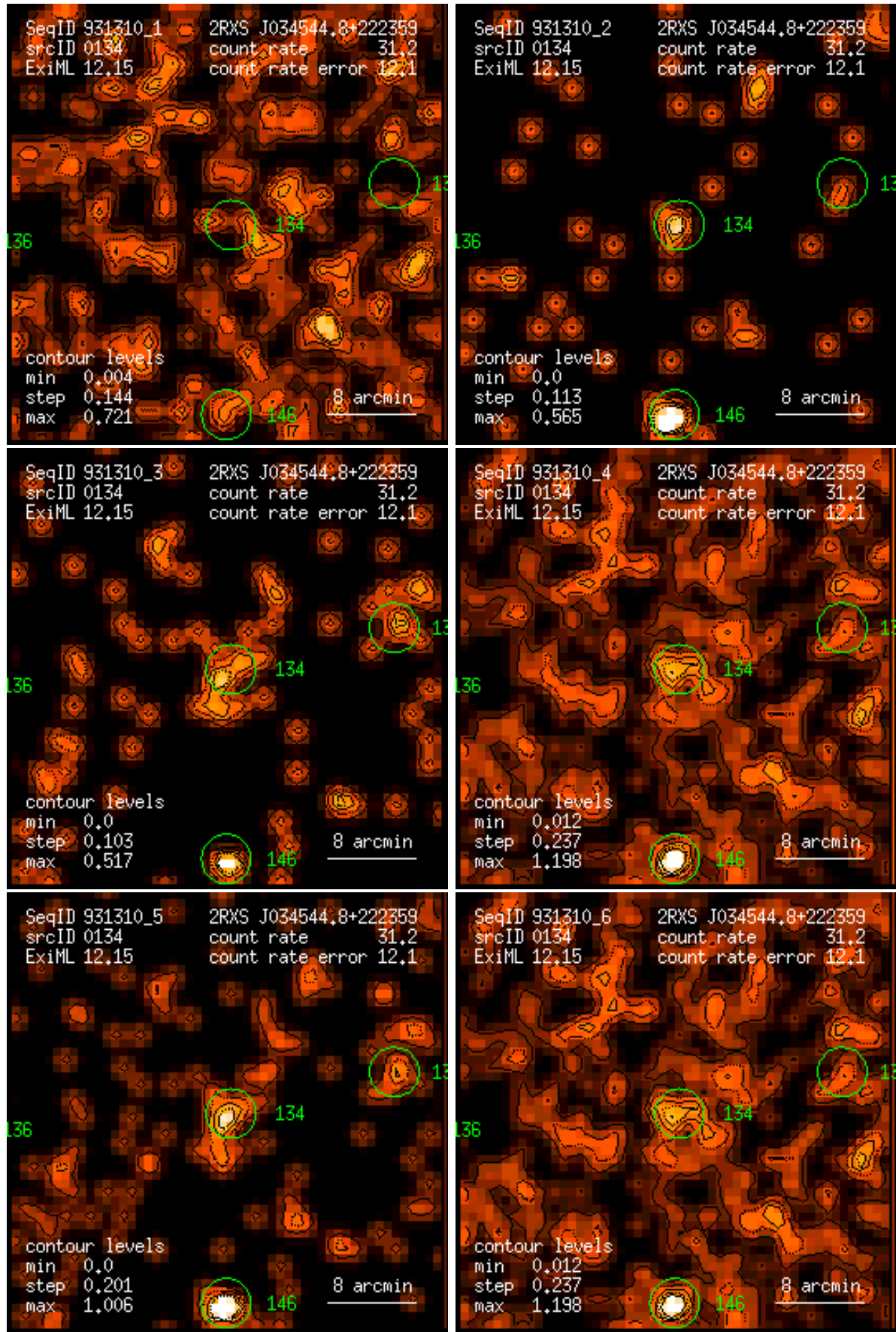
Figure 134: RASS 931310: detection 0134: band rate images, Gaussian filter: (1) PSPC channels 11 – 41, (2) 52 – 90, (3) 91 – 201, (4) 11 – 235, (5) 52 – 201, (6) 11 – 201. Broad band rates in counts/ks. Band rate contour levels in counts/ks/arcmin 2 .
