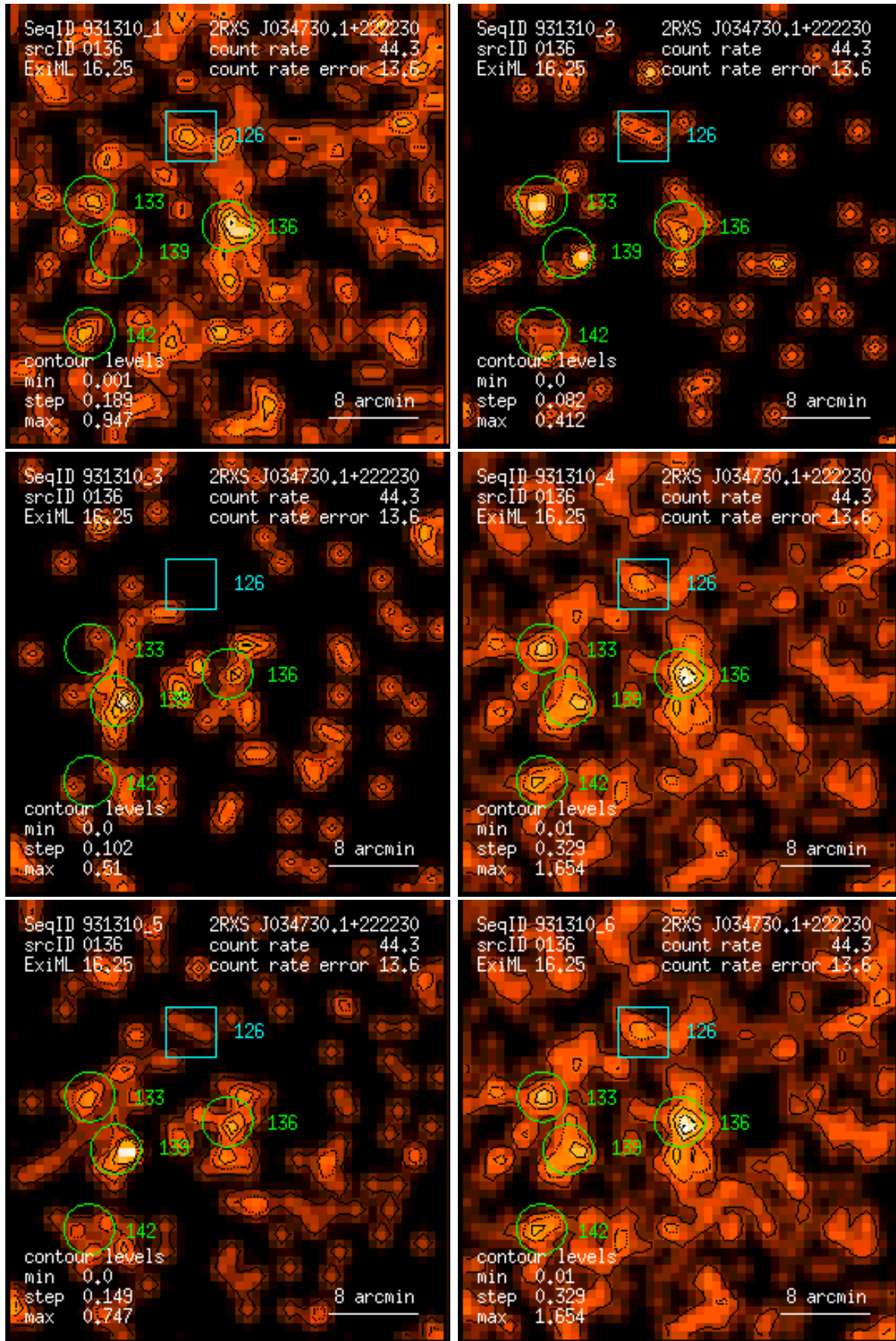
Figure 136: RASS 931310: detection 0136: band rate images, Gaussian filter: (1) PSPC channels 11 – 41, (2) 52 – 90, (3) 91 – 201, (4) 11 – 235, (5) 52 – 201, (6) 11 – 201. Broad band rates in counts/ks. Band rate contour levels in counts/ks/arcmin 2 .
