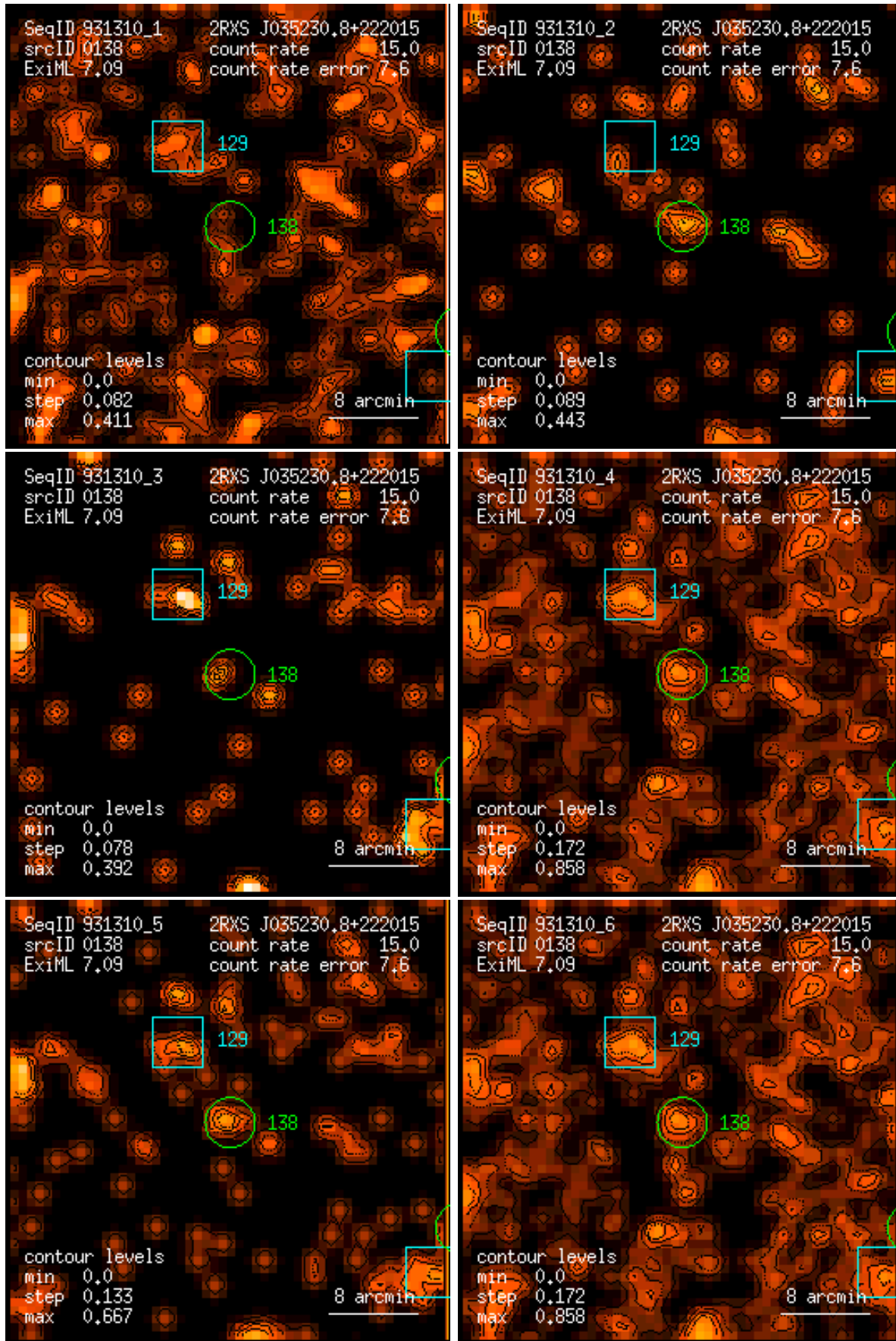
Figure 138: RASS 931310: detection 0138: band rate images, Gaussian filter: (1) PSPC channels 11 – 41, (2) 52 – 90, (3) 91 – 201, (4) 11 – 235, (5) 52 – 201, (6) 11 – 201. Broad band rates in counts/ks. Band rate contour levels in counts/ks/arcmin 2 .
