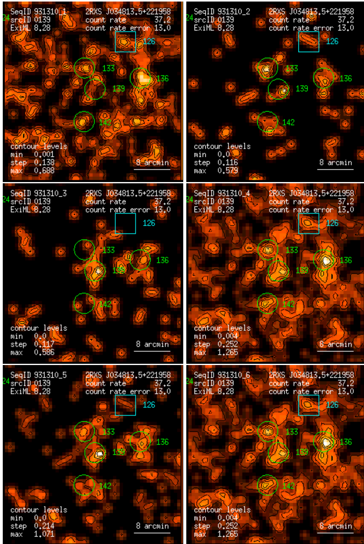
Figure 139: RASS 931310: detection 0139: band rate images, Gaussian filter: (1) PSPC channels 11 – 41, (2) 52 – 90, (3) 91 – 201, (4) 11 – 235, (5) 52 – 201, (6) 11 – 201. Broad band rates in counts/ks. Band rate contour levels in counts/ks/arcmin 2 .
