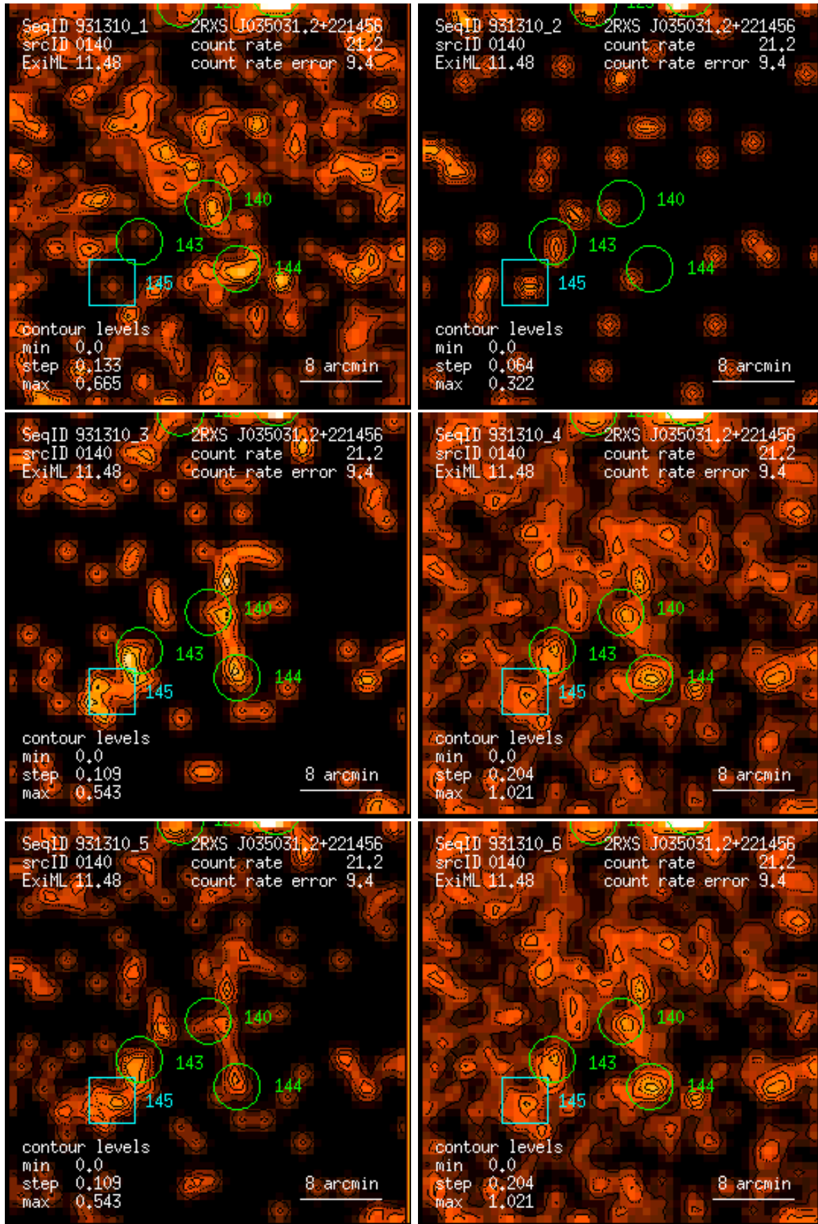
Figure 140: RASS 931310: detection 0140: band rate images, Gaussian filter: (1) PSPC channels 11 – 41, (2) 52 – 90, (3) 91 – 201, (4) 11 – 235, (5) 52 – 201, (6) 11 – 201. Broad band rates in counts/ks. Band rate contour levels in counts/ks/arcmin 2 .
