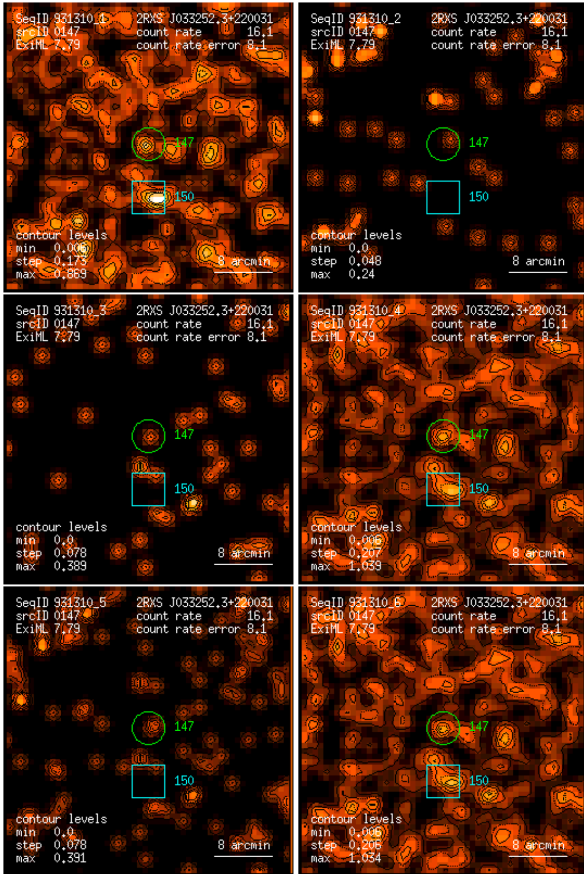
Figure 147: RASS 931310: detection 0147: band rate images, Gaussian filter: (1) PSPC channels 11 – 41, (2) 52 – 90, (3) 91 – 201, (4) 11 – 235, (5) 52 – 201, (6) 11 – 201. Broad band rates in counts/ks. Band rate contour levels in counts/ks/arcmin 2 .
