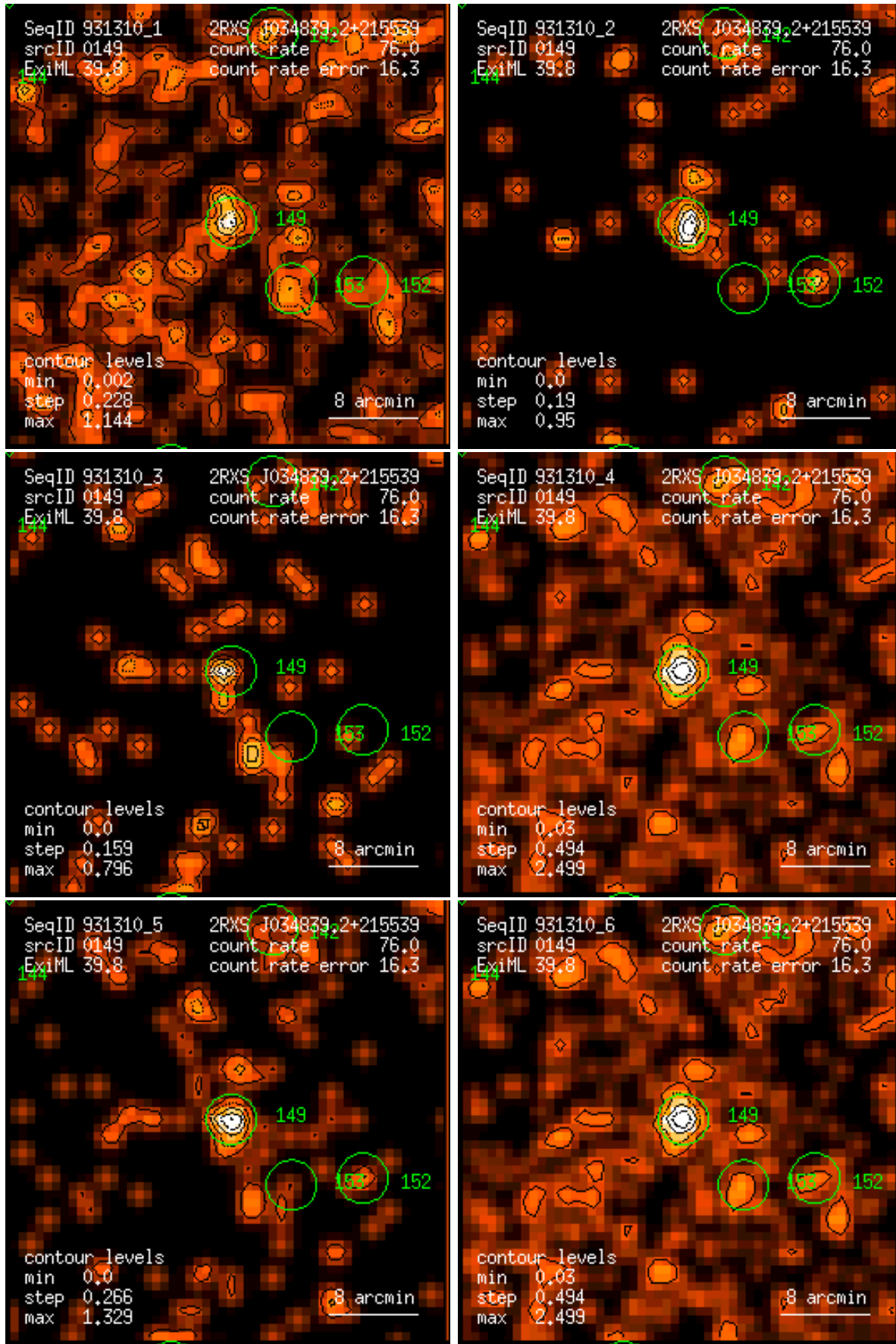
Figure 149: RASS 931310: detection 0149: band rate images, Gaussian filter: (1) PSPC channels 11 – 41, (2) 52 – 90, (3) 91 – 201, (4) 11 – 235, (5) 52 – 201, (6) 11 – 201. Broad band rates in counts/ks. Band rate contour levels in counts/ks/arcmin 2 .
