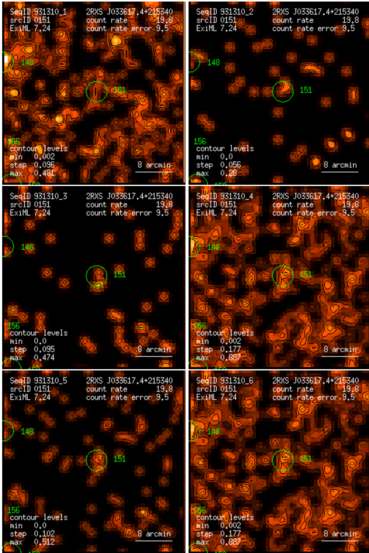
Figure 151: RASS 931310: detection 0151: band rate images, Gaussian filter: (1) PSPC channels 11 – 41, (2) 52 – 90, (3) 91 – 201, (4) 11 – 235, (5) 52 – 201, (6) 11 – 201. Broad band rates in counts/ks. Band rate contour levels in counts/ks/arcmin 2 .
