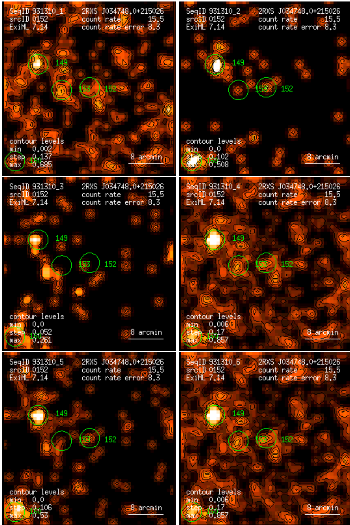
Figure 152: RASS 931310: detection 0152: band rate images, Gaussian filter: (1) PSPC channels 11 – 41, (2) 52 – 90, (3) 91 – 201, (4) 11 – 235, (5) 52 – 201, (6) 11 – 201. Broad band rates in counts/ks. Band rate contour levels in counts/ks/arcmin 2 .
