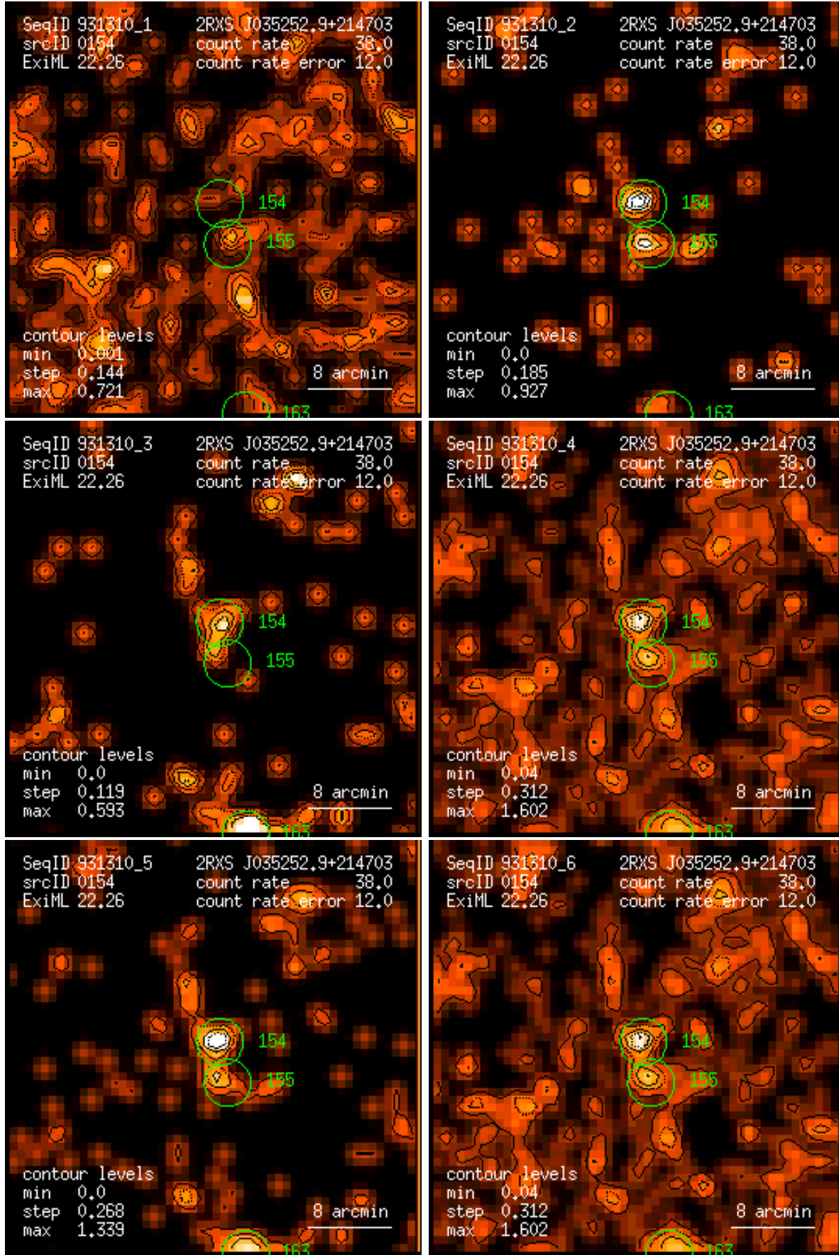
Figure 154: RASS 931310: detection 0154: band rate images, Gaussian filter: (1) PSPC channels 11 – 41, (2) 52 – 90, (3) 91 – 201, (4) 11 – 235, (5) 52 – 201, (6) 11 – 201. Broad band rates in counts/ks. Band rate contour levels in counts/ks/arcmin 2 .
