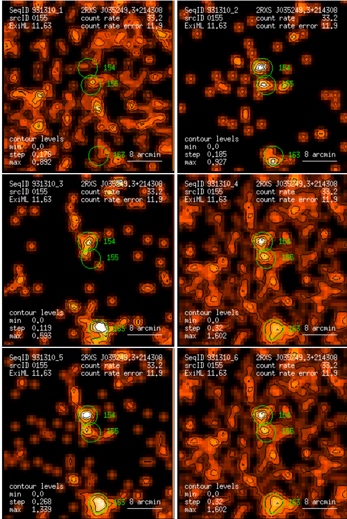
Figure 155: RASS 931310: detection 0155: band rate images, Gaussian filter: (1) PSPC channels 11 – 41, (2) 52 – 90, (3) 91 – 201, (4) 11 – 235, (5) 52 – 201, (6) 11 – 201. Broad band rates in counts/ks. Band rate contour levels in counts/ks/arcmin 2 .
