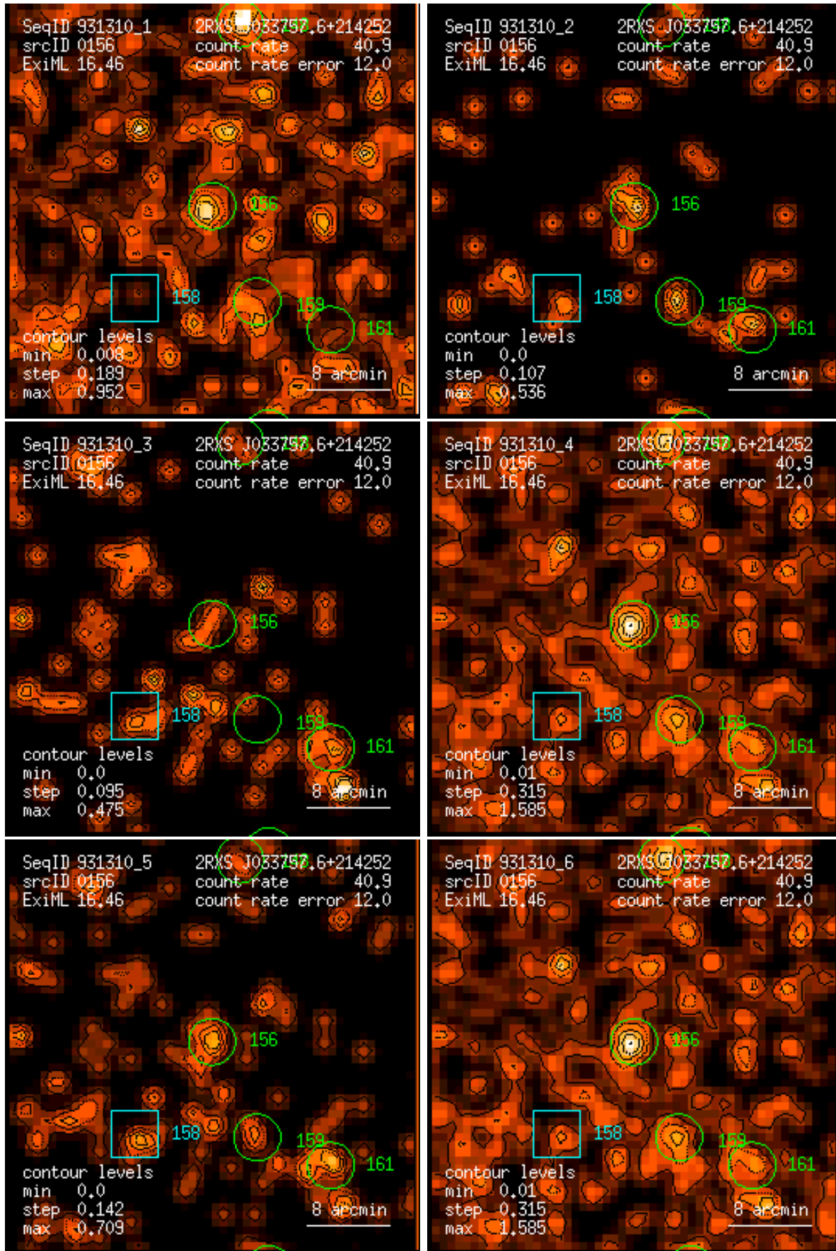
Figure 156: RASS 931310: detection 0156: band rate images, Gaussian filter: (1) PSPC channels 11 – 41, (2) 52 – 90, (3) 91 – 201, (4) 11 – 235, (5) 52 – 201, (6) 11 – 201. Broad band rates in counts/ks. Band rate contour levels in counts/ks/arcmin 2 .
