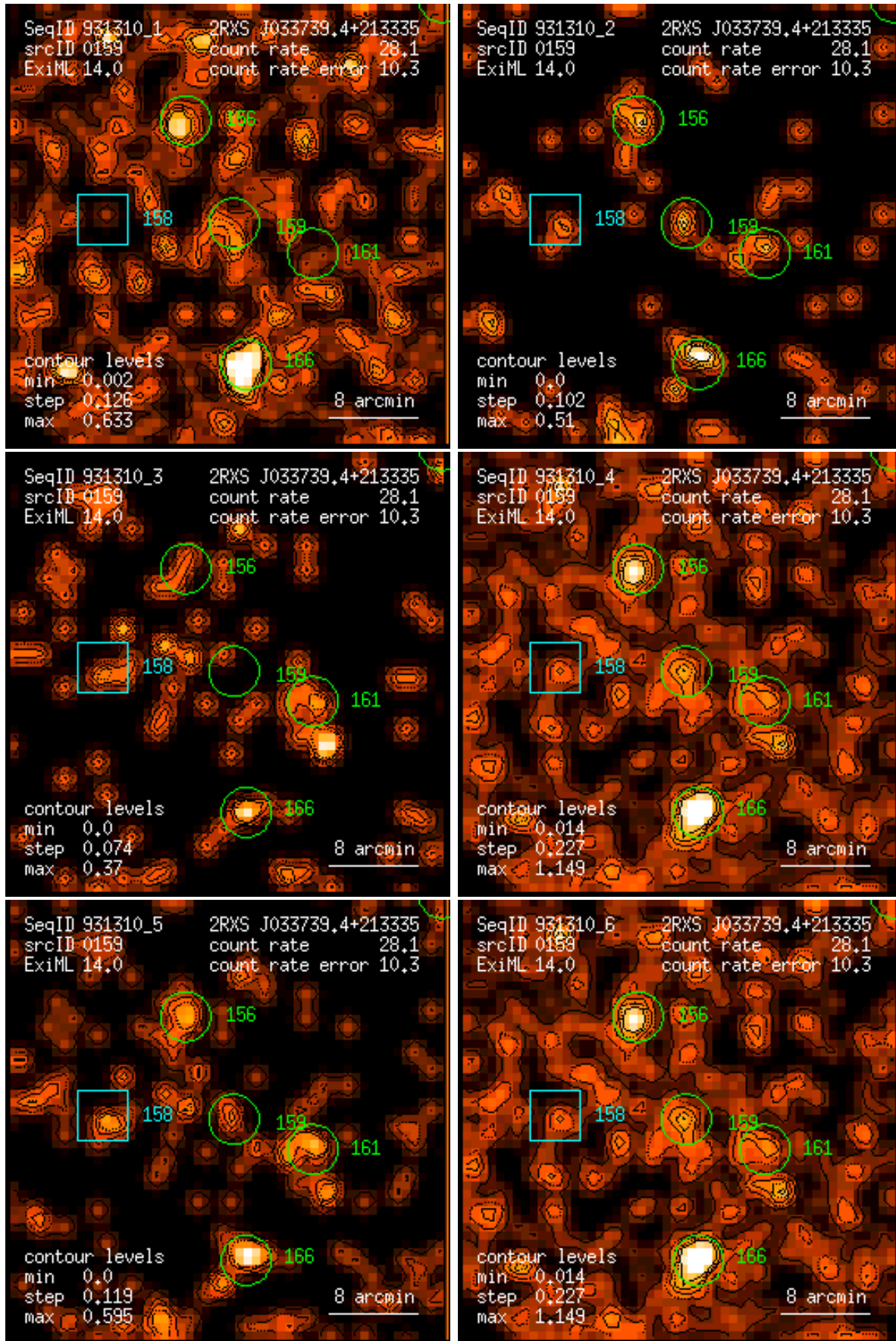
Figure 159: RASS 931310: detection 0159: band rate images, Gaussian filter: (1) PSPC channels 11 – 41, (2) 52 – 90, (3) 91 – 201, (4) 11 – 235, (5) 52 – 201, (6) 11 – 201. Broad band rates in counts/ks. Band rate contour levels in counts/ks/arcmin 2 .
