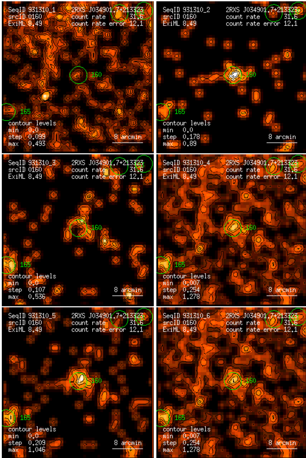
Figure 160: RASS 931310: detection 0160: band rate images, Gaussian filter: (1) PSPC channels 11 – 41, (2) 52 – 90, (3) 91 – 201, (4) 11 – 235, (5) 52 – 201, (6) 11 – 201. Broad band rates in counts/ks. Band rate contour levels in counts/ks/arcmin 2 .
