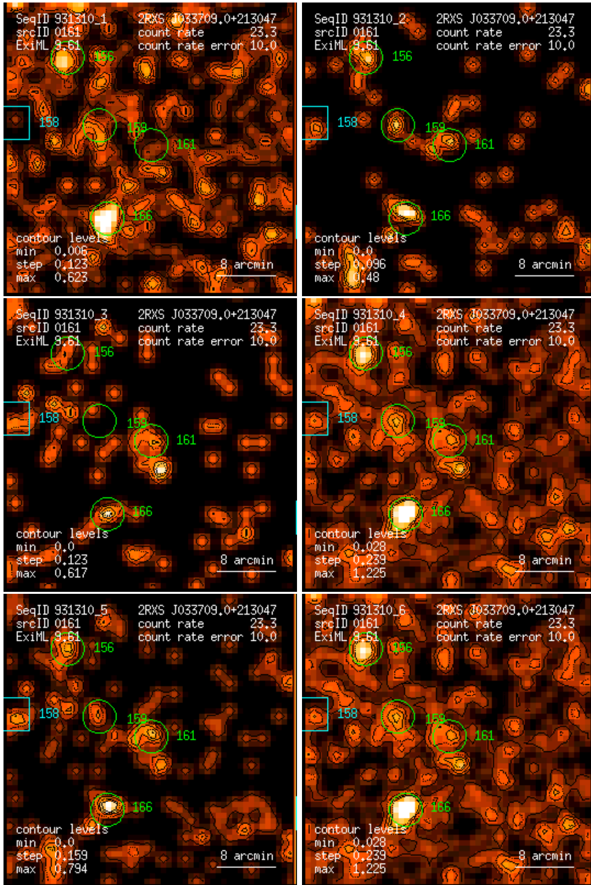
Figure 161: RASS 931310: detection 0161: band rate images, Gaussian filter: (1) PSPC channels 11 – 41, (2) 52 – 90, (3) 91 – 201, (4) 11 – 235, (5) 52 – 201, (6) 11 – 201. Broad band rates in counts/ks. Band rate contour levels in counts/ks/arcmin 2 .
