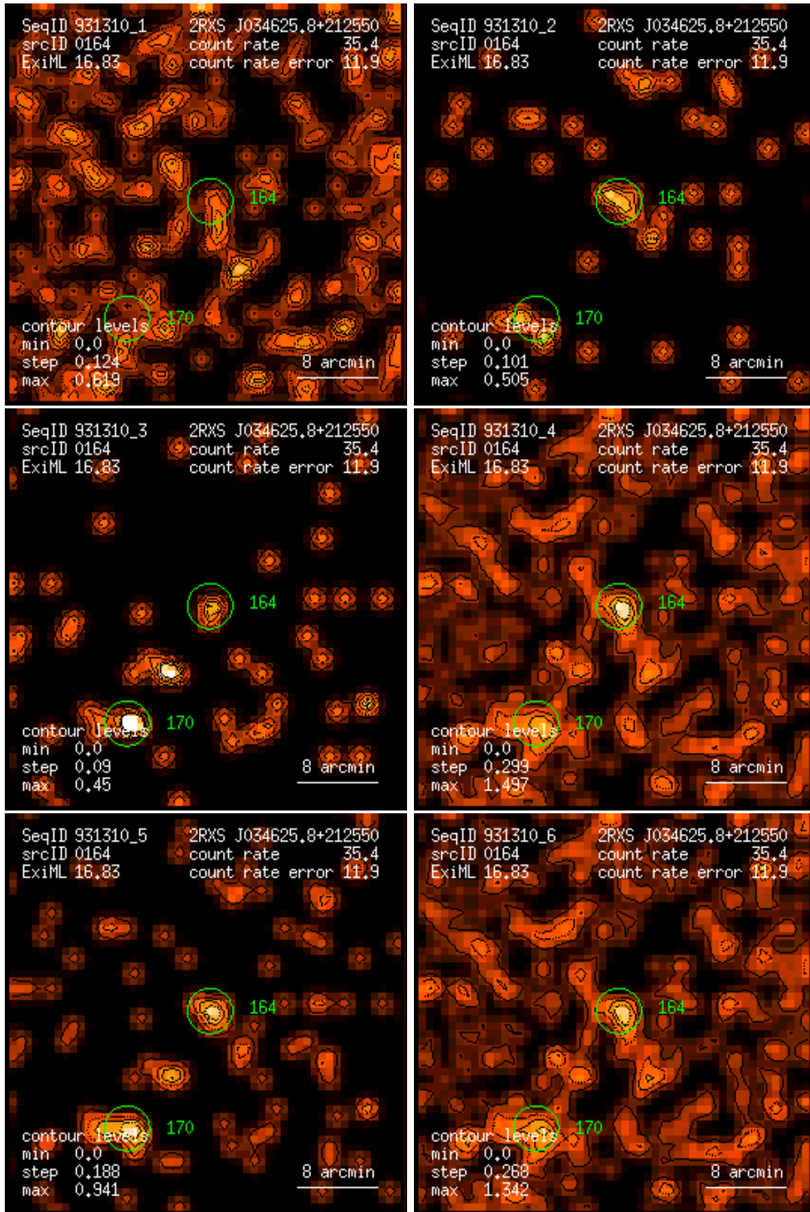
Figure 164: RASS 931310: detection 0164: band rate images, Gaussian filter: (1) PSPC channels 11 – 41, (2) 52 – 90, (3) 91 – 201, (4) 11 – 235, (5) 52 – 201, (6) 11 – 201. Broad band rates in counts/ks. Band rate contour levels in counts/ks/arcmin 2 .
