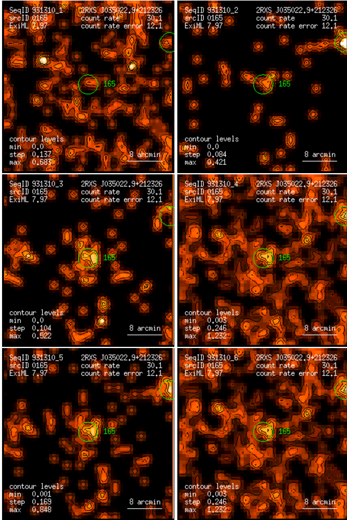
Figure 165: RASS 931310: detection 0165: band rate images, Gaussian filter: (1) PSPC channels 11 – 41, (2) 52 – 90, (3) 91 – 201, (4) 11 – 235, (5) 52 – 201, (6) 11 – 201. Broad band rates in counts/ks. Band rate contour levels in counts/ks/arcmin 2 .
