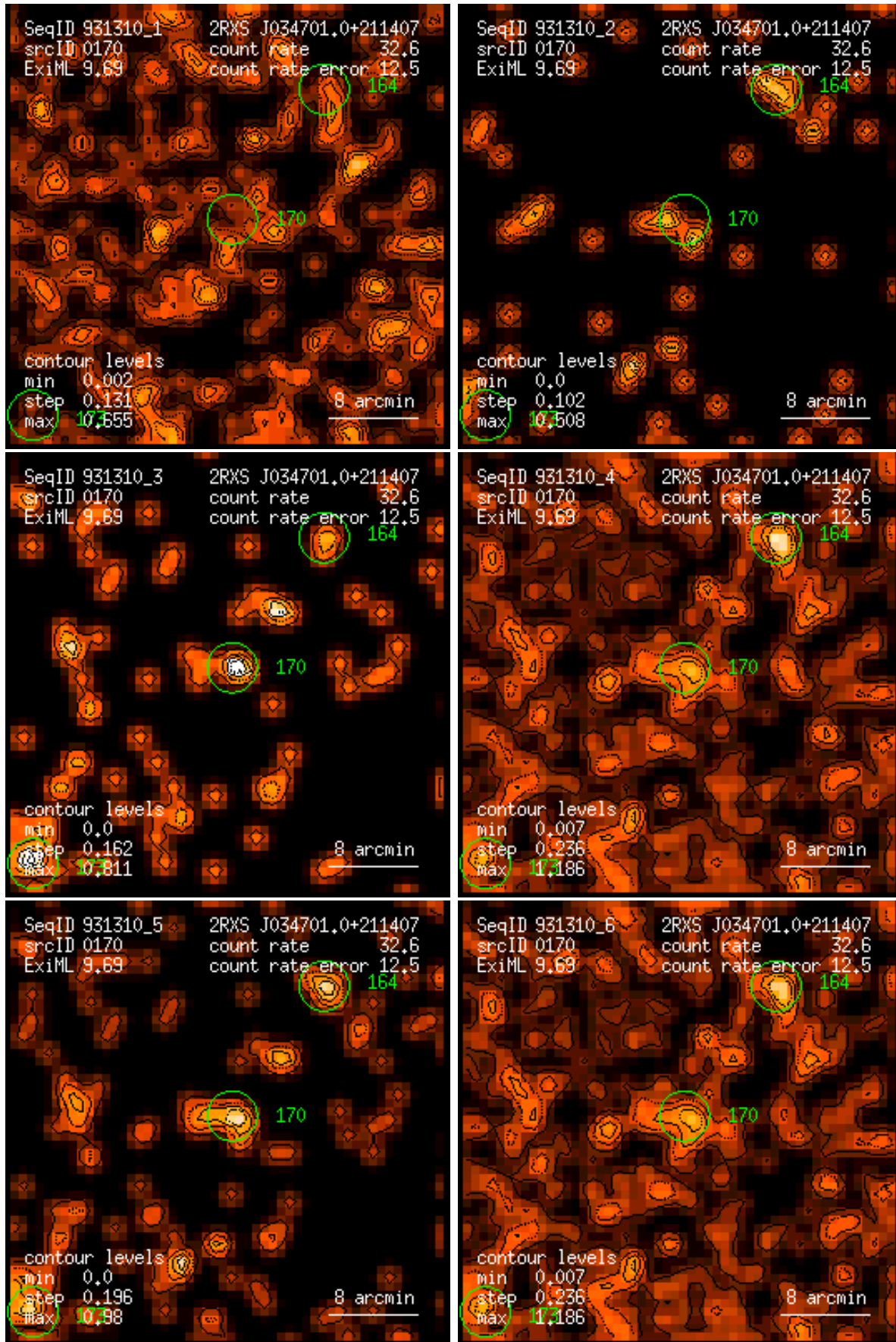
Figure 170: RASS 931310: detection 0170: band rate images, Gaussian filter: (1) PSPC channels 11 – 41, (2) 52 – 90, (3) 91 – 201, (4) 11 – 235, (5) 52 – 201, (6) 11 – 201. Broad band rates in counts/ks. Band rate contour levels in counts/ks/arcmin 2 .
