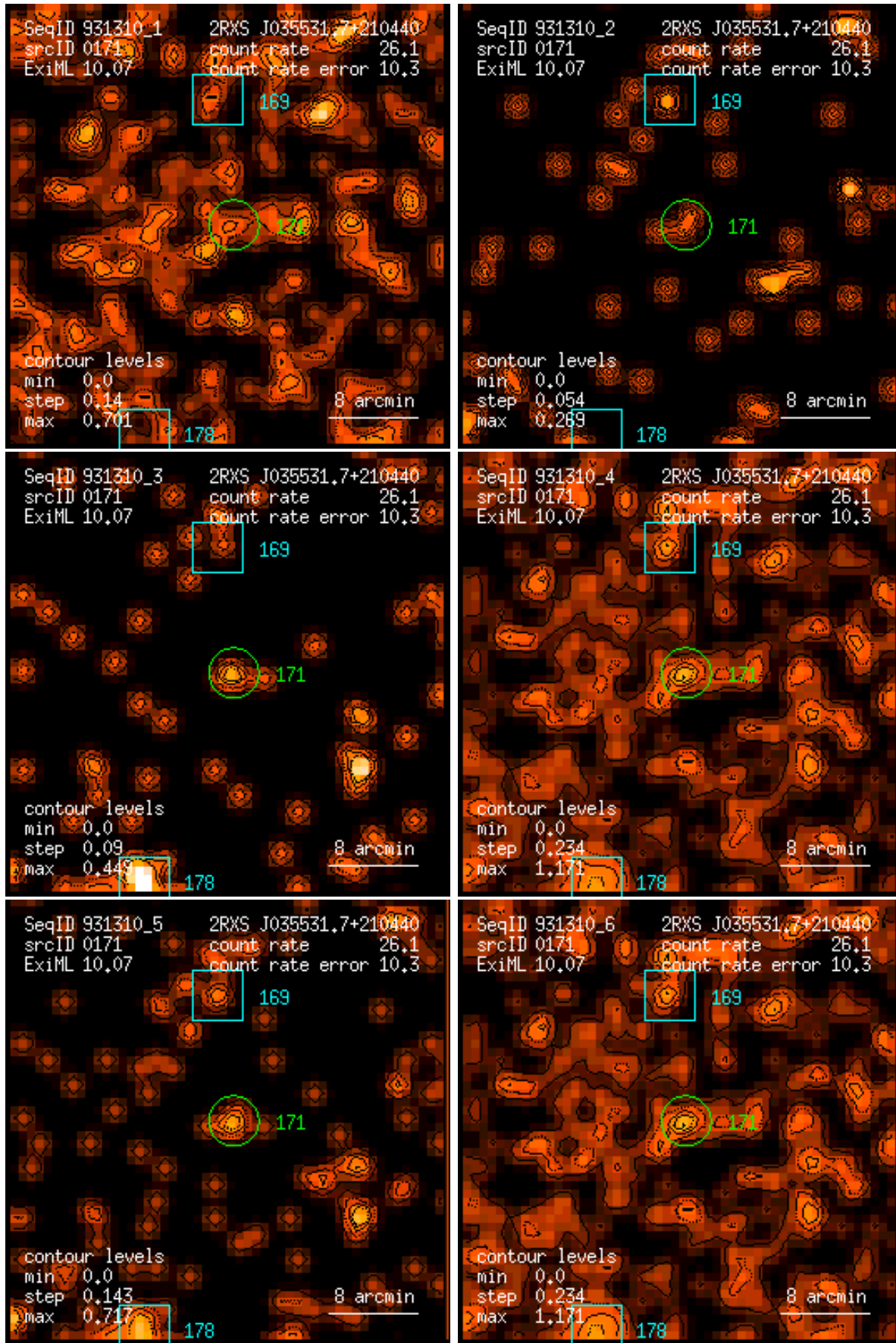
Figure 171: RASS 931310: detection 0171: band rate images, Gaussian filter: (1) PSPC channels 11 – 41, (2) 52 – 90, (3) 91 – 201, (4) 11 – 235, (5) 52 – 201, (6) 11 – 201. Broad band rates in counts/ks. Band rate contour levels in counts/ks/arcmin 2 .
