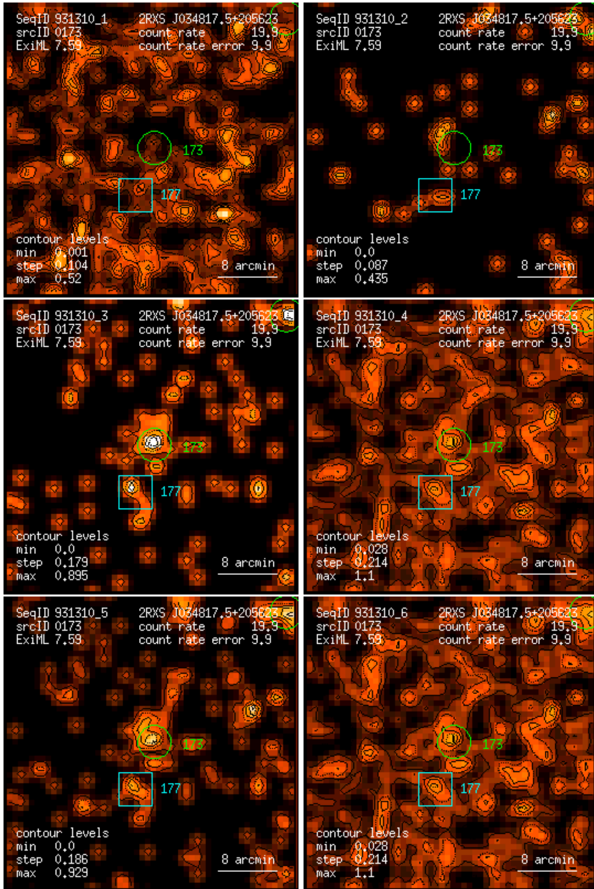
Figure 173: RASS 931310: detection 0173: band rate images, Gaussian filter: (1) PSPC channels 11 – 41, (2) 52 – 90, (3) 91 – 201, (4) 11 – 235, (5) 52 – 201, (6) 11 – 201. Broad band rates in counts/ks. Band rate contour levels in counts/ks/arcmin 2 .
