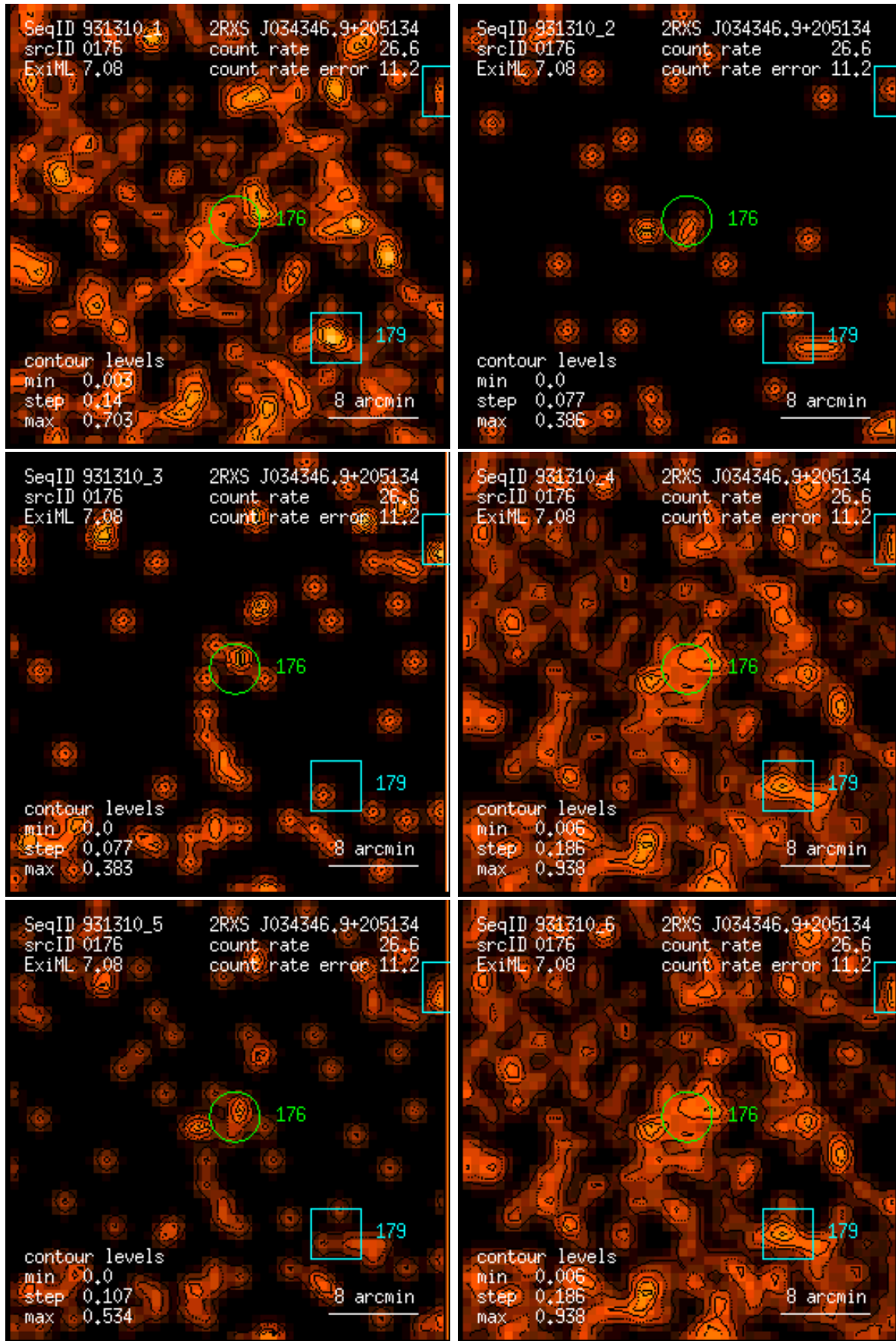
Figure 176: RASS 931310: detection 0176: band rate images, Gaussian filter: (1) PSPC channels 11 – 41, (2) 52 – 90, (3) 91 – 201, (4) 11 – 235, (5) 52 – 201, (6) 11 – 201. Broad band rates in counts/ks. Band rate contour levels in counts/ks/arcmin 2 .
