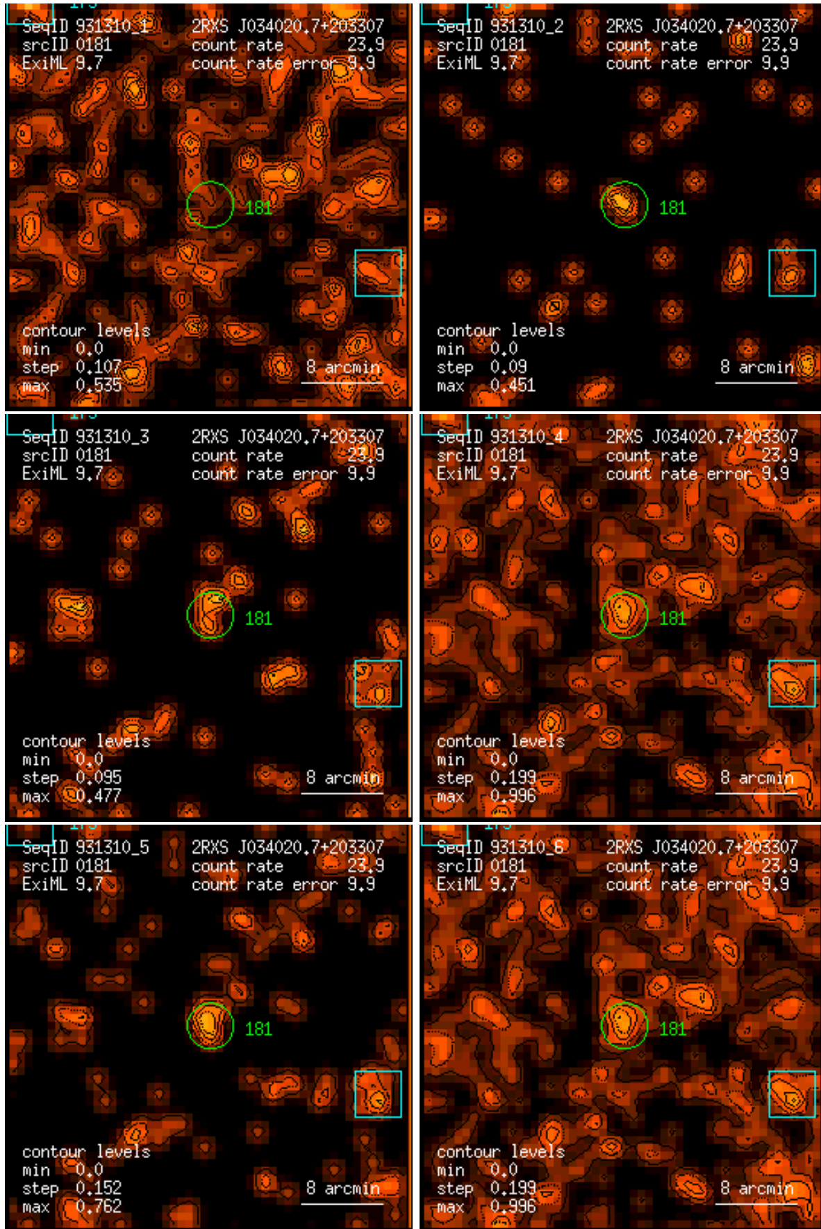
Figure 181: RASS 931310: detection 0181: band rate images, Gaussian filter: (1) PSPC channels 11 – 41, (2) 52 – 90, (3) 91 – 201, (4) 11 – 235, (5) 52 – 201, (6) 11 – 201. Broad band rates in counts/ks. Band rate contour levels in counts/ks/arcmin 2 .
