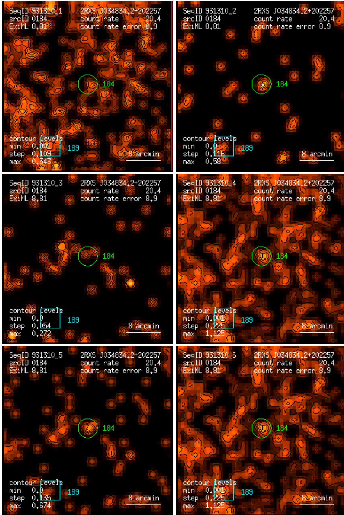
Figure 184: RASS 931310: detection 0184: band rate images, Gaussian filter: (1) PSPC channels 11 – 41, (2) 52 – 90, (3) 91 – 201, (4) 11 – 235, (5) 52 – 201, (6) 11 – 201. Broad band rates in counts/ks. Band rate contour levels in counts/ks/arcmin 2 .
