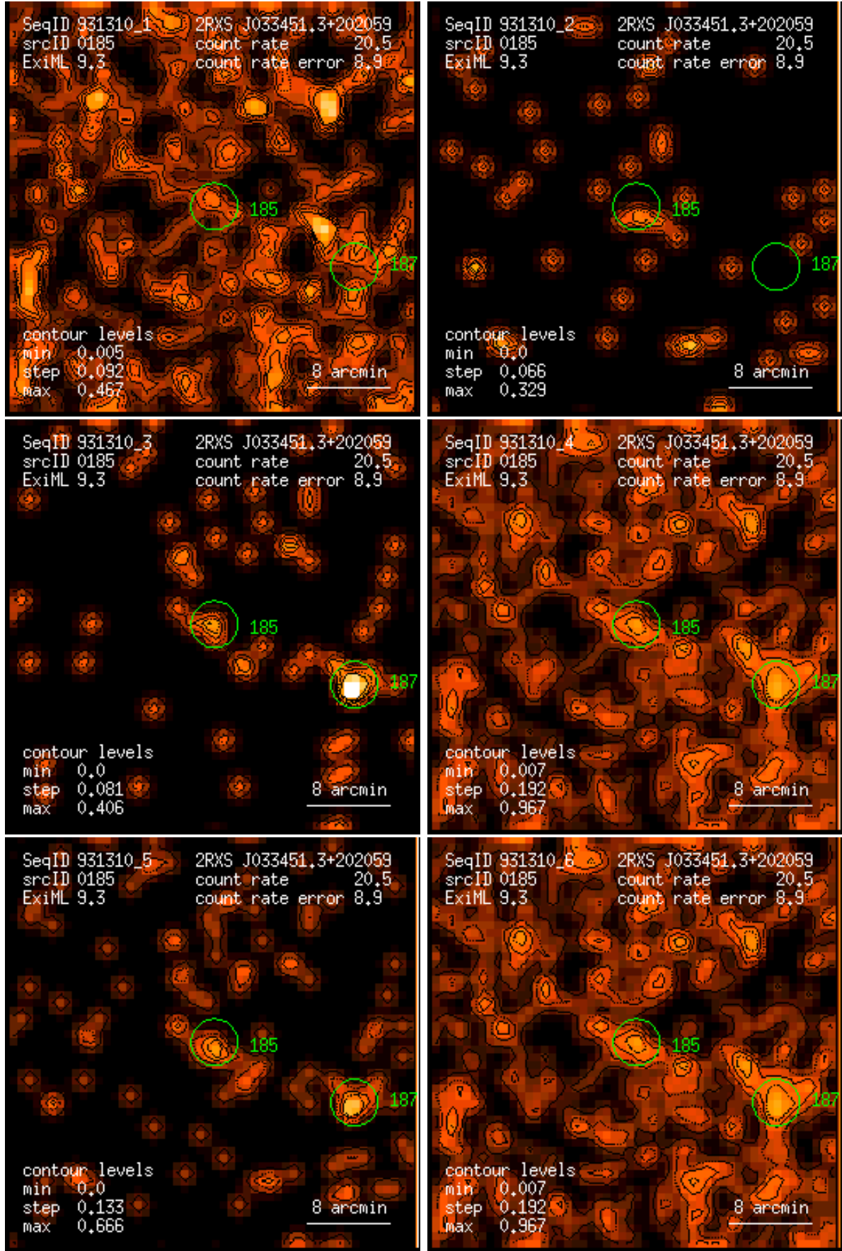
Figure 185: RASS 931310: detection 0185: band rate images, Gaussian filter: (1) PSPC channels 11 – 41, (2) 52 – 90, (3) 91 – 201, (4) 11 – 235, (5) 52 – 201, (6) 11 – 201. Broad band rates in counts/ks. Band rate contour levels in counts/ks/arcmin 2 .
