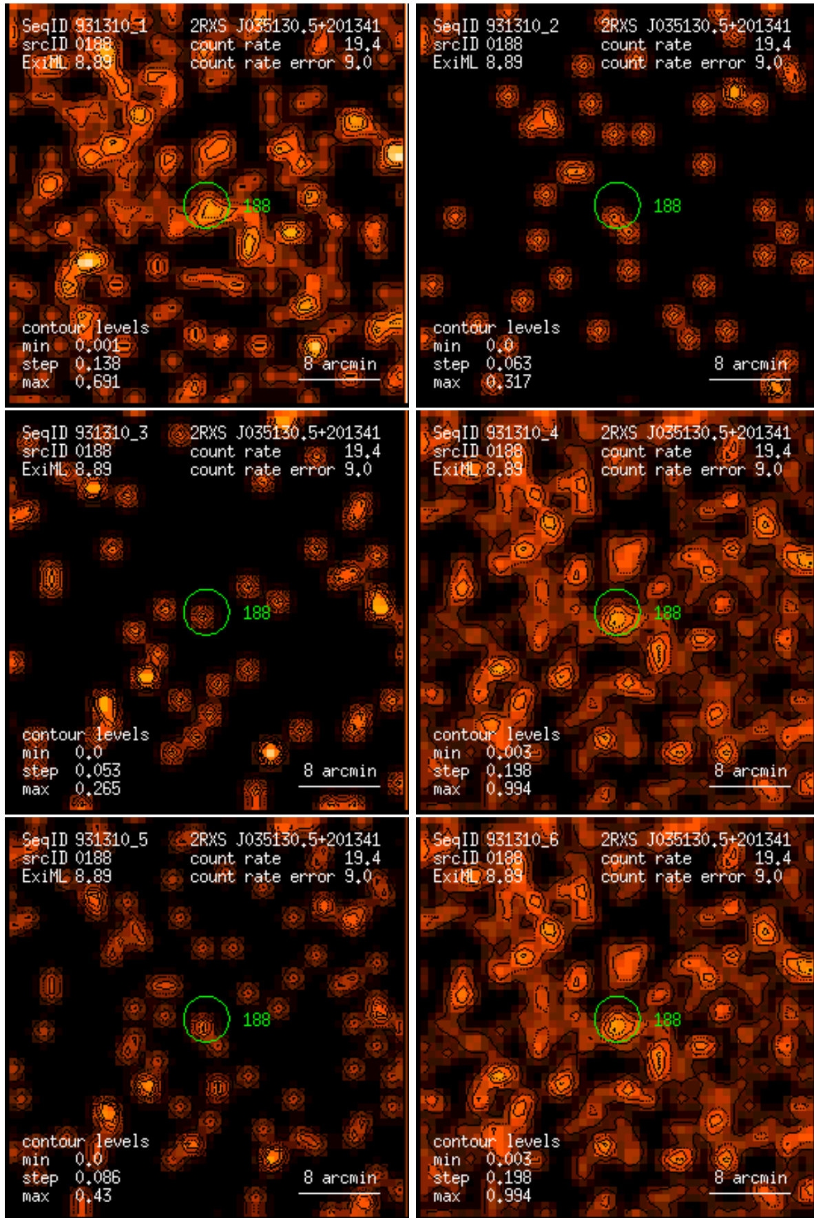
Figure 188: RASS 931310: detection 0188: band rate images, Gaussian filter: (1) PSPC channels 11 – 41, (2) 52 – 90, (3) 91 – 201, (4) 11 – 235, (5) 52 – 201, (6) 11 – 201. Broad band rates in counts/ks. Band rate contour levels in counts/ks/arcmin 2 .
