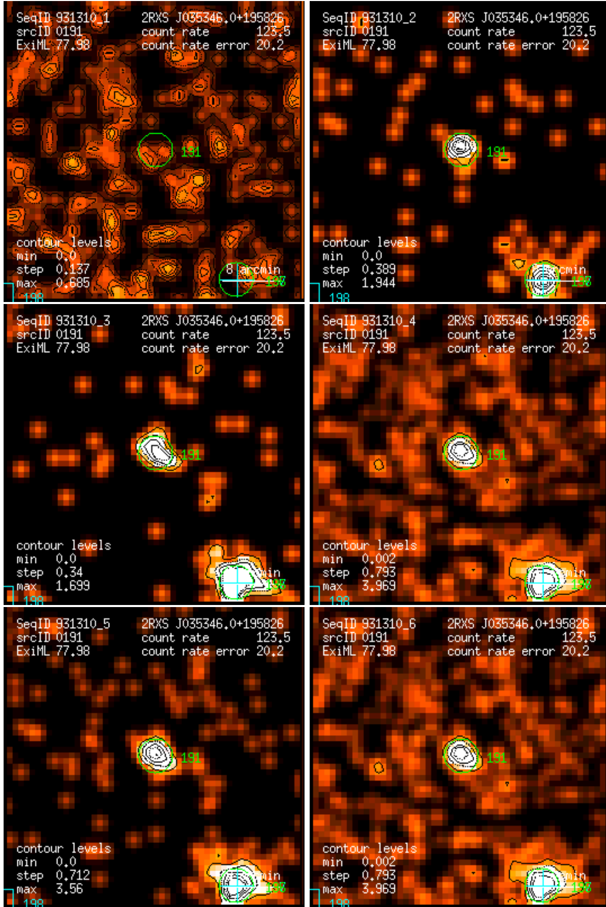
Figure 191: RASS 931310: detection 0191: band rate images, Gaussian filter: (1) PSPC channels 11 – 41, (2) 52 – 90, (3) 91 – 201, (4) 11 – 235, (5) 52 – 201, (6) 11 – 201. Broad band rates in counts/ks. Band rate contour levels in counts/ks/arcmin 2 .
