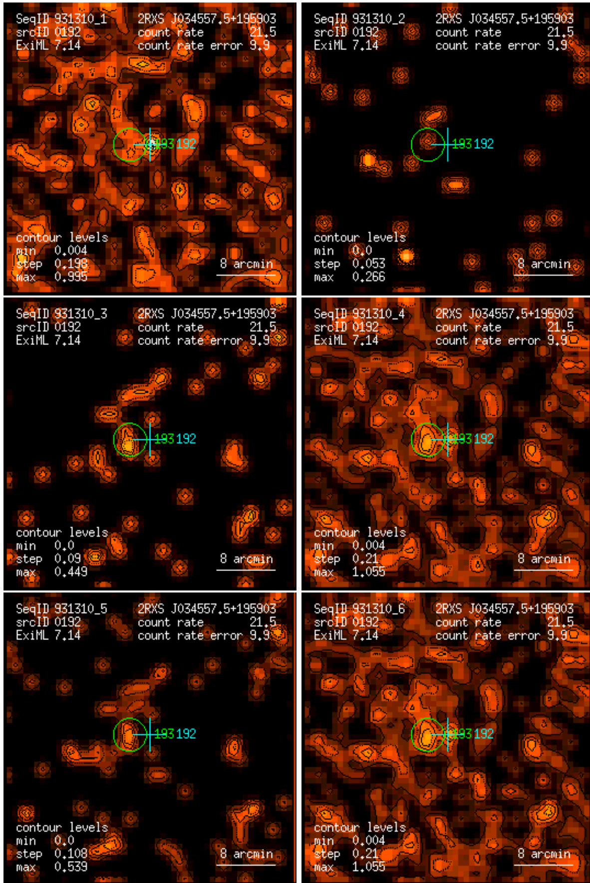
Figure 192: RASS 931310: detection 0192: band rate images, Gaussian filter: (1) PSPC channels 11 – 41, (2) 52 – 90, (3) 91 – 201, (4) 11 – 235, (5) 52 – 201, (6) 11 – 201. Broad band rates in counts/ks. Band rate contour levels in counts/ks/arcmin 2 .
