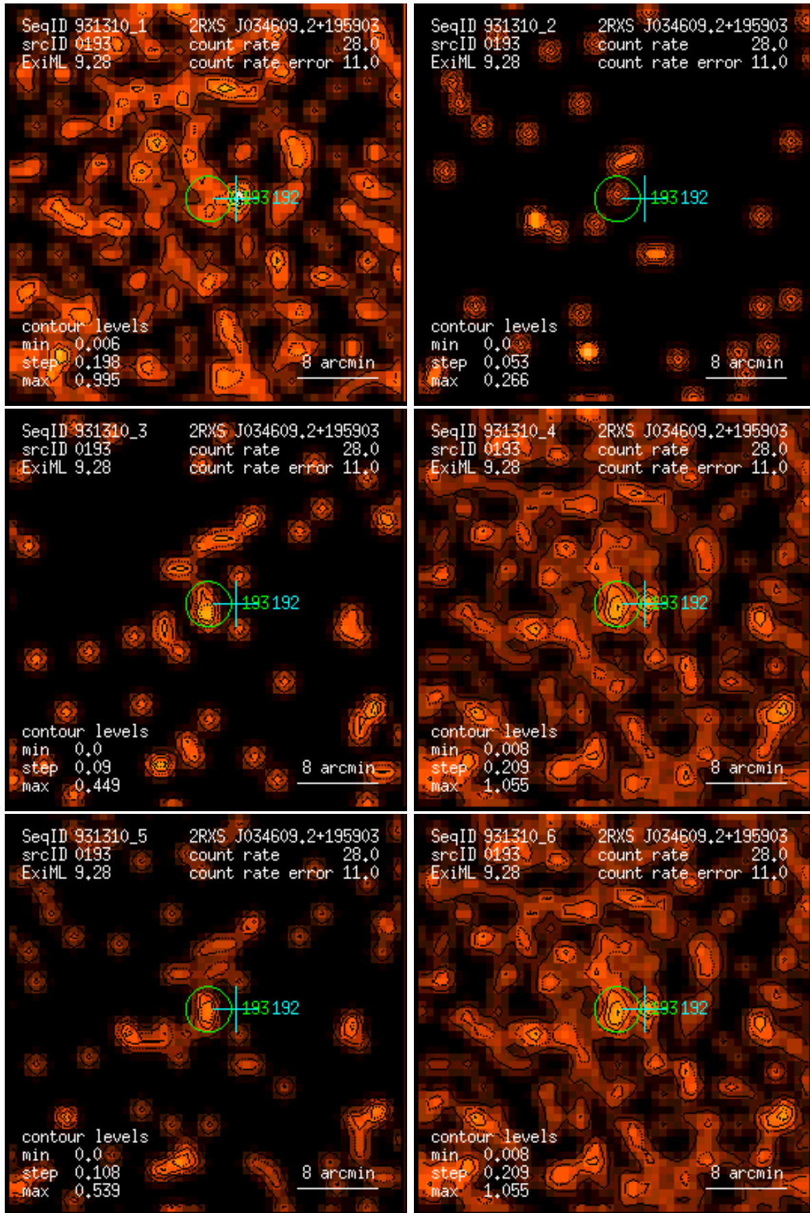
Figure 193: RASS 931310: detection 0193: band rate images, Gaussian filter: (1) PSPC channels 11 – 41, (2) 52 – 90, (3) 91 – 201, (4) 11 – 235, (5) 52 – 201, (6) 11 – 201. Broad band rates in counts/ks. Band rate contour levels in counts/ks/arcmin 2 .
