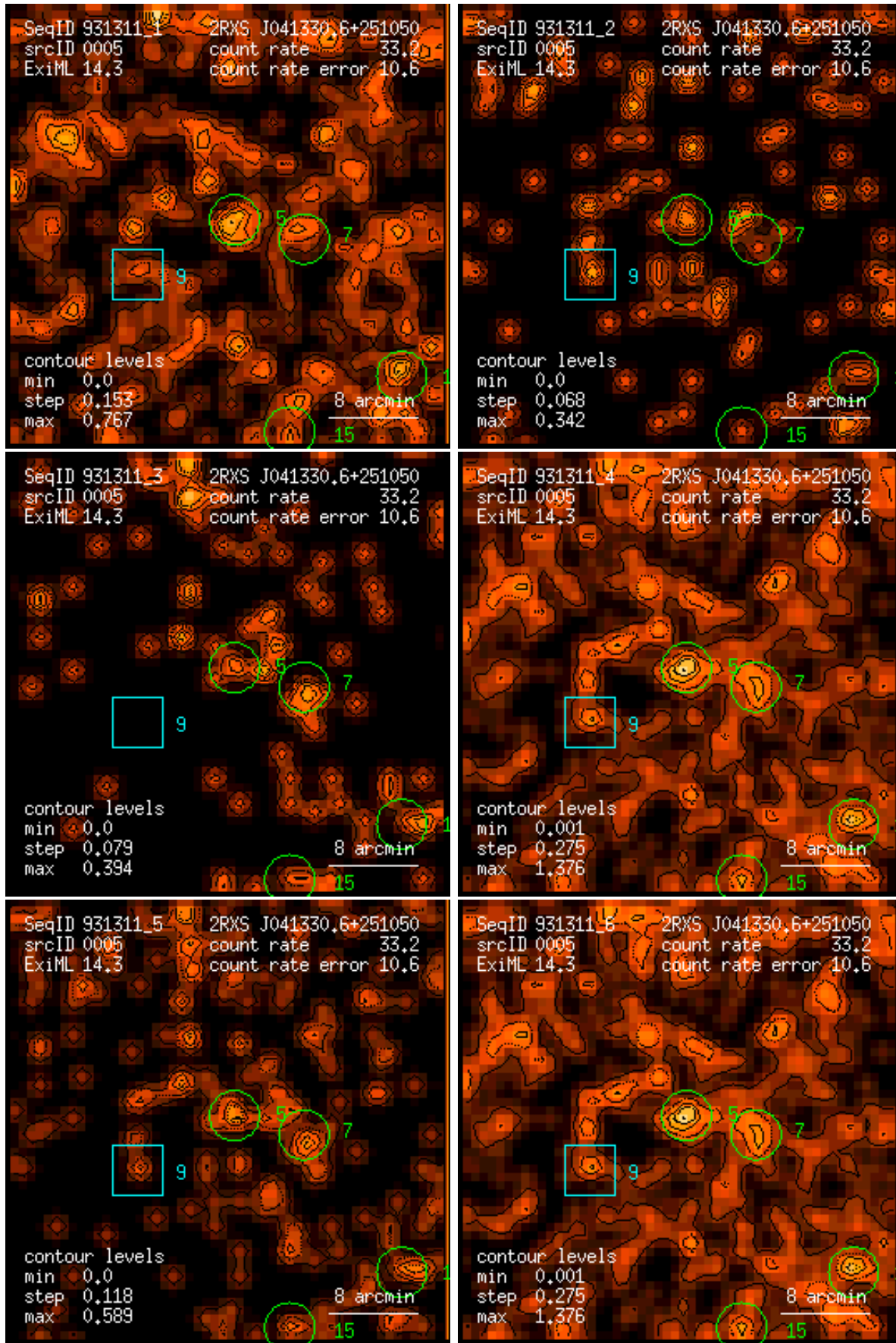
Figure 5: RASS 931311: detection 0005: band rate images, Gaussian filter: (1) PSPC channels 11 – 41, (2) 52 – 90, (3) 91 – 201, (4) 11 – 235, (5) 52 – 201, (6) 11 – 201. Broad band rates in counts/ks. Band rate contour levels in counts/ks/arcmin 2 .
