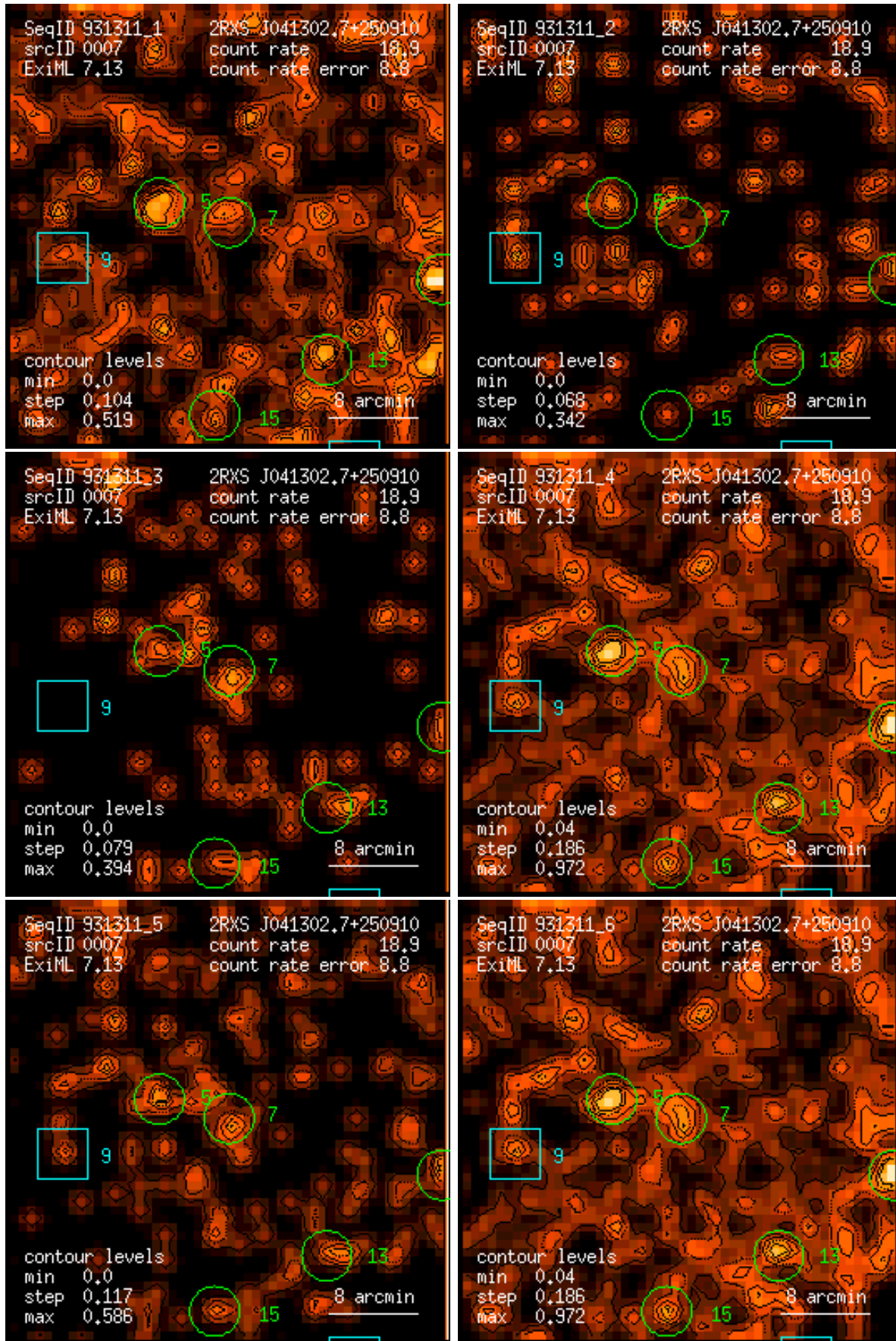
Figure 7: RASS 931311: detection 0007: band rate images, Gaussian filter: (1) PSPC channels 11 – 41, (2) 52 – 90, (3) 91 – 201, (4) 11 – 235, (5) 52 – 201, (6) 11 – 201. Broad band rates in counts/ks. Band rate contour levels in counts/ks/arcmin 2 .
