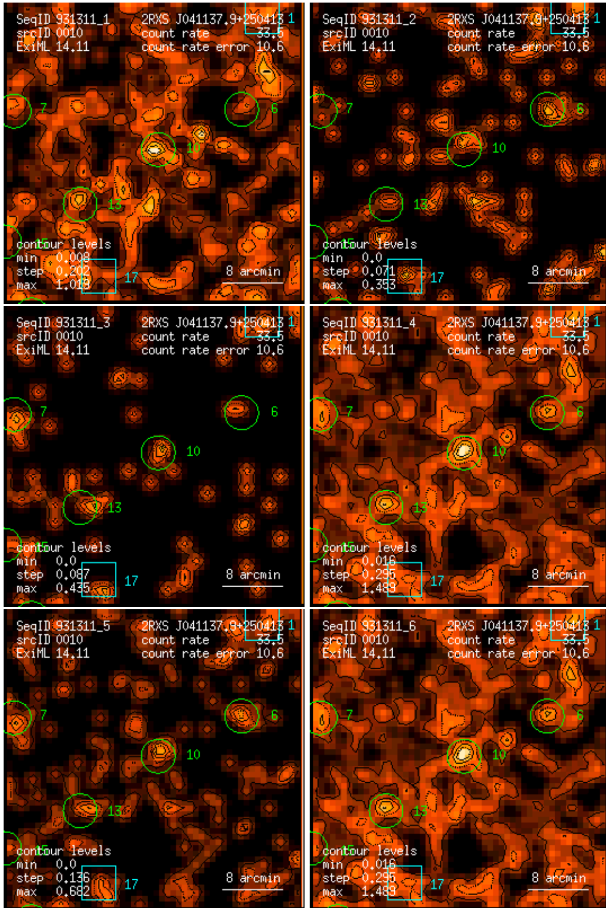
Figure 10: RASS 931311: detection 0010: band rate images, Gaussian filter: (1) PSPC channels 11 – 41, (2) 52 – 90, (3) 91 – 201, (4) 11 – 235, (5) 52 – 201, (6) 11 – 201. Broad band rates in counts/ks. Band rate contour levels in counts/ks/arcmin 2 .
