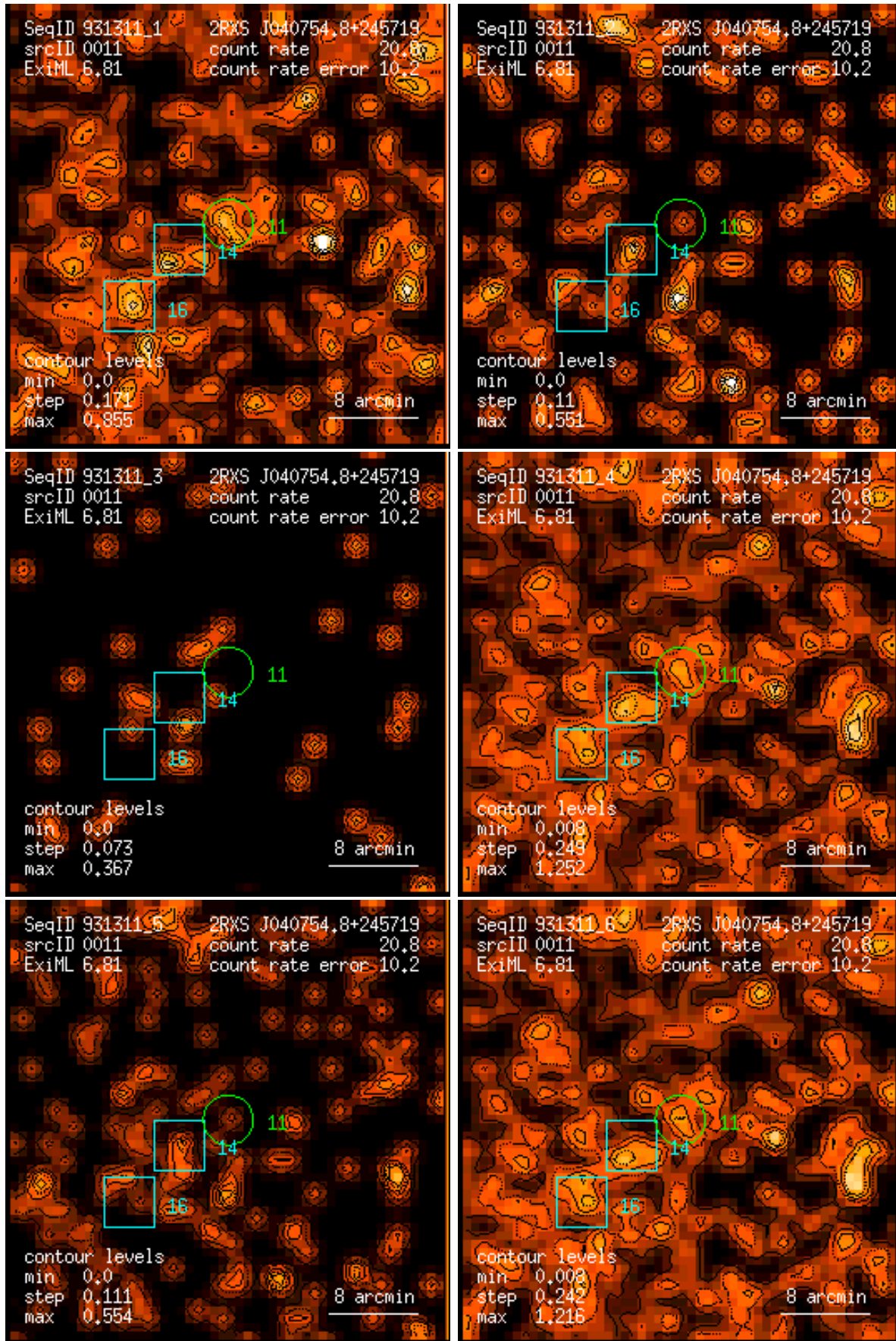
Figure 11: RASS 931311: detection 0011: band rate images, Gaussian filter: (1) PSPC channels 11 – 41, (2) 52 – 90, (3) 91 – 201, (4) 11 – 235, (5) 52 – 201, (6) 11 – 201. Broad band rates in counts/ks. Band rate contour levels in counts/ks/arcmin 2 .
