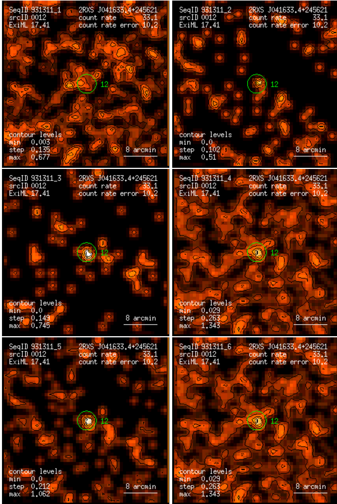
Figure 12: RASS 931311: detection 0012: band rate images, Gaussian filter: (1) PSPC channels 11 – 41, (2) 52 – 90, (3) 91 – 201, (4) 11 – 235, (5) 52 – 201, (6) 11 – 201. Broad band rates in counts/ks. Band rate contour levels in counts/ks/arcmin 2 .
