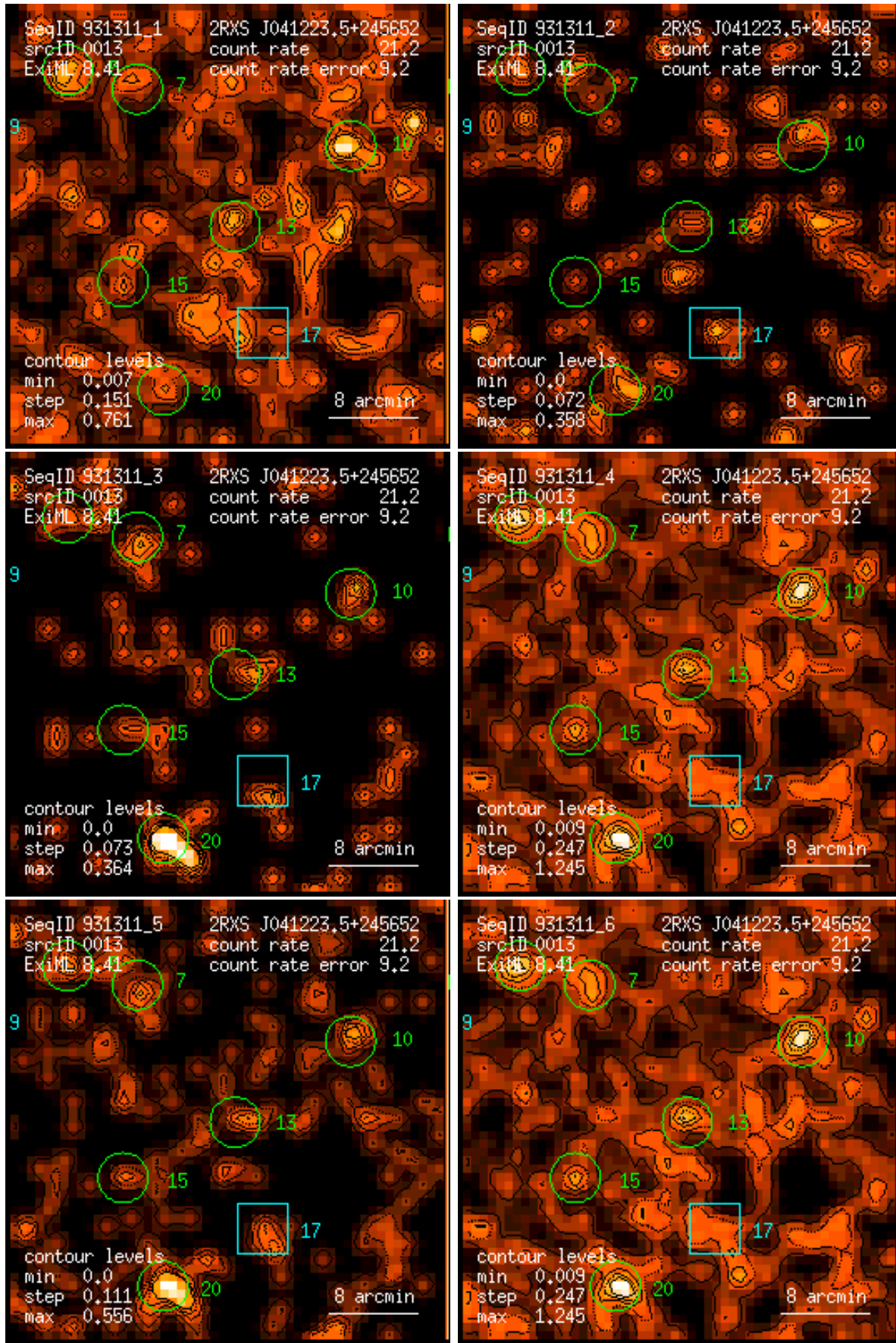
Figure 13: RASS 931311: detection 0013: band rate images, Gaussian filter: (1) PSPC channels 11 – 41, (2) 52 – 90, (3) 91 – 201, (4) 11 – 235, (5) 52 – 201, (6) 11 – 201. Broad band rates in counts/ks. Band rate contour levels in counts/ks/arcmin 2 .
