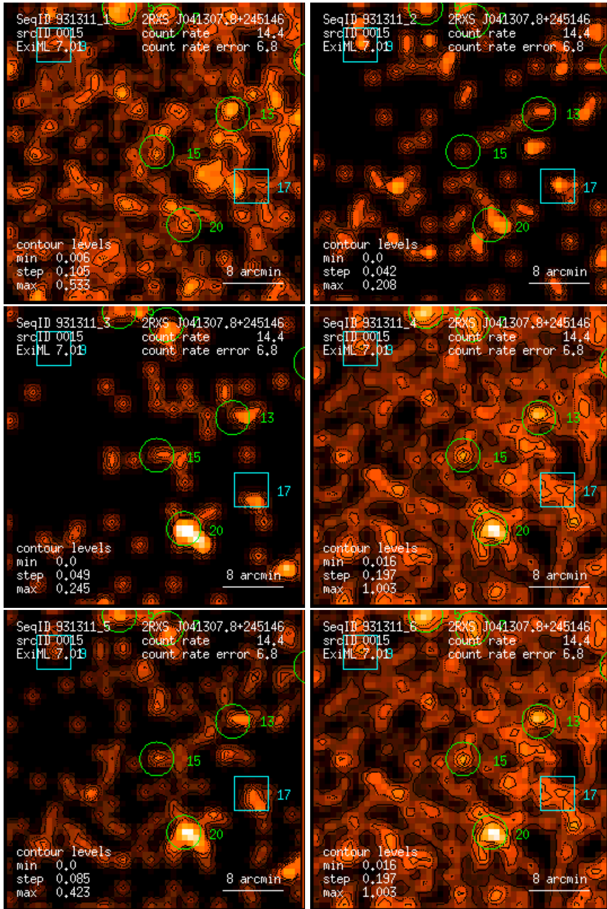
Figure 15: RASS 931311: detection 0015: band rate images, Gaussian filter: (1) PSPC channels 11 – 41, (2) 52 – 90, (3) 91 – 201, (4) 11 – 235, (5) 52 – 201, (6) 11 – 201. Broad band rates in counts/ks. Band rate contour levels in counts/ks/arcmin 2 .
