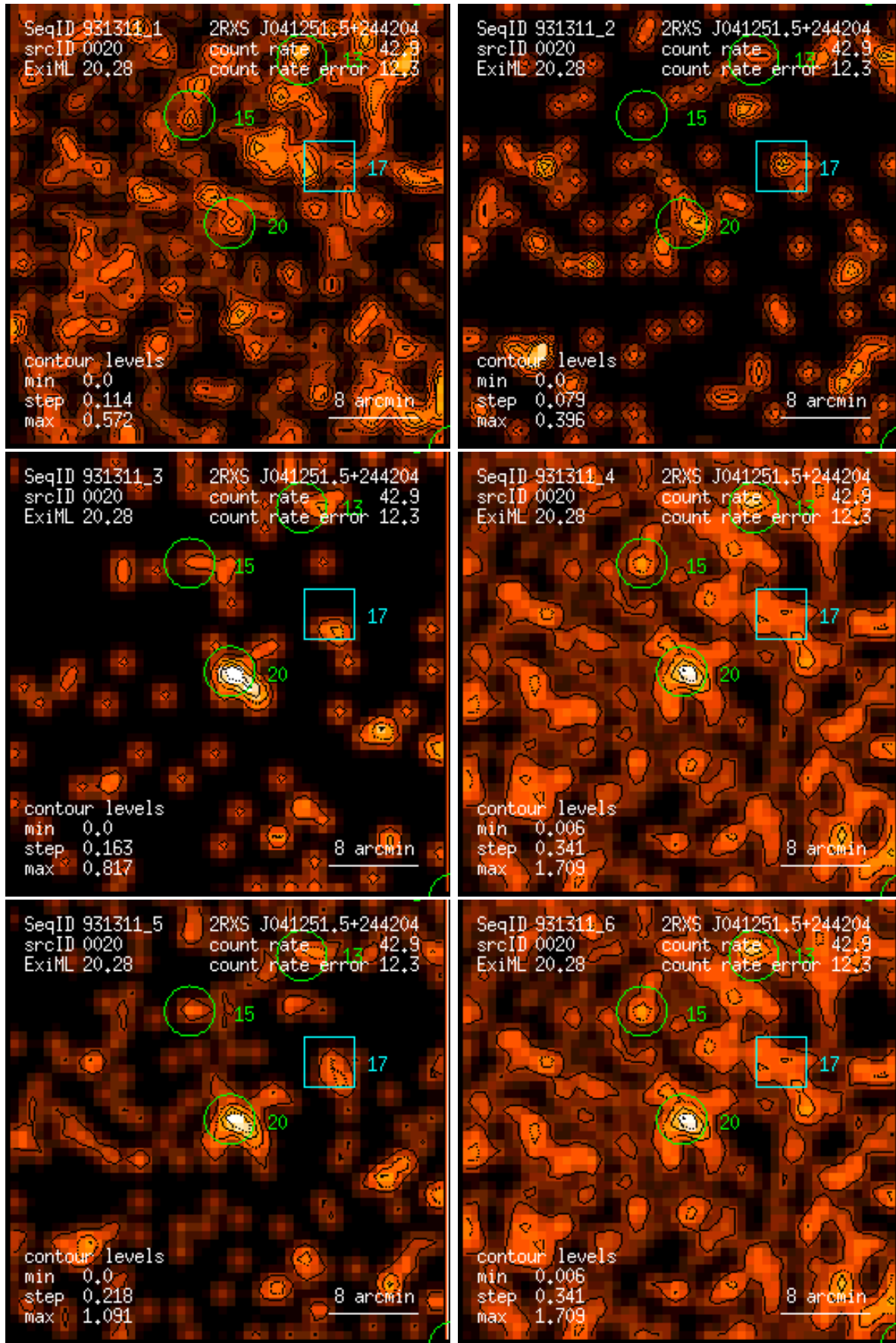
Figure 20: RASS 931311: detection 0020: band rate images, Gaussian filter: (1) PSPC channels 11 – 41, (2) 52 – 90, (3) 91 – 201, (4) 11 – 235, (5) 52 – 201, (6) 11 – 201. Broad band rates in counts/ks. Band rate contour levels in counts/ks/arcmin 2 .
