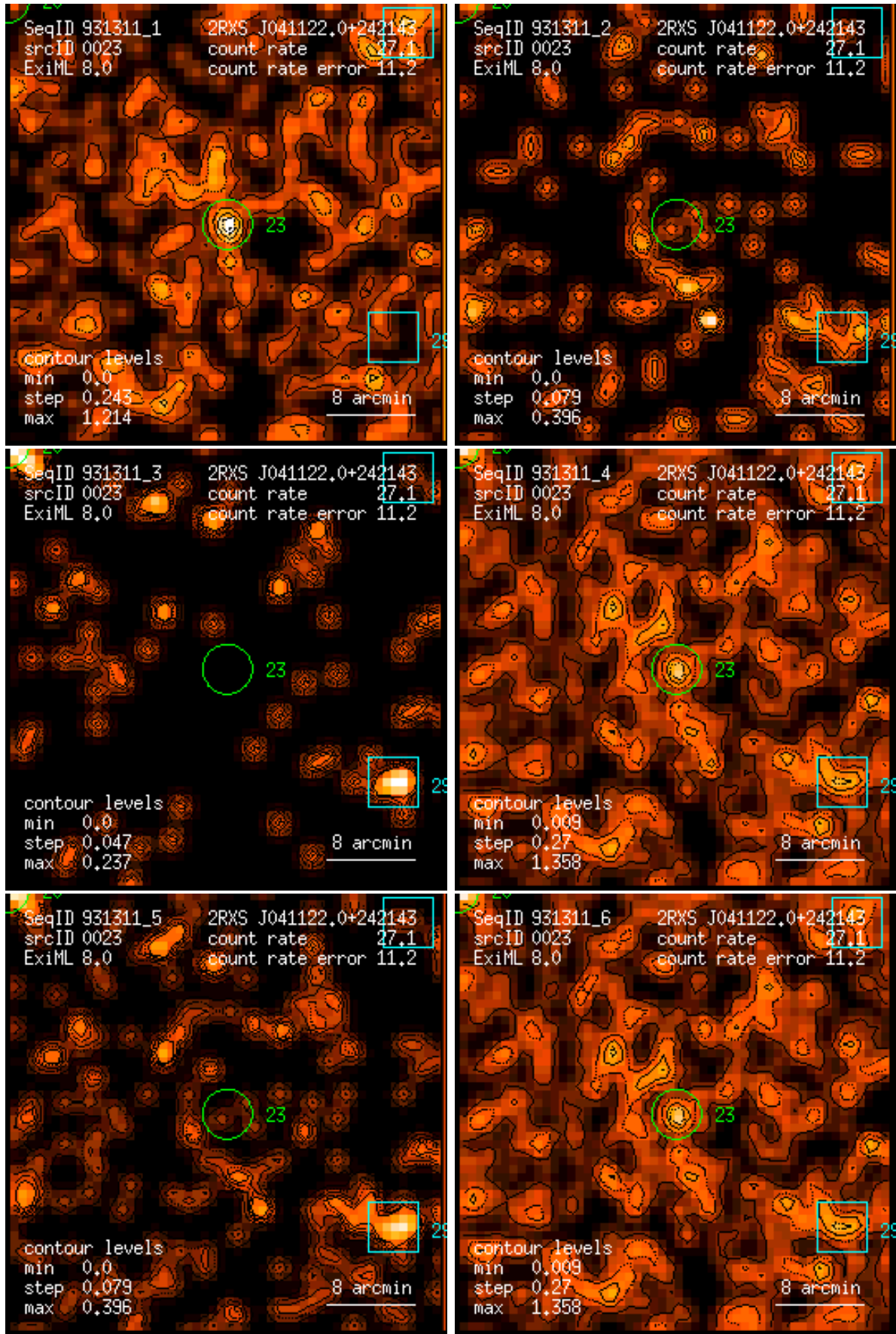
Figure 23: RASS 931311: detection 0023: band rate images, Gaussian filter: (1) PSPC channels 11 – 41, (2) 52 – 90, (3) 91 – 201, (4) 11 – 235, (5) 52 – 201, (6) 11 – 201. Broad band rates in counts/ks. Band rate contour levels in counts/ks/arcmin 2 .
