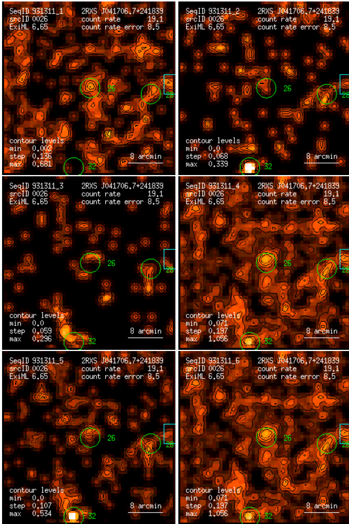
Figure 26: RASS 931311: detection 0026: band rate images, Gaussian filter: (1) PSPC channels 11 – 41, (2) 52 – 90, (3) 91 – 201, (4) 11 – 235, (5) 52 – 201, (6) 11 – 201. Broad band rates in counts/ks. Band rate contour levels in counts/ks/arcmin 2 .
