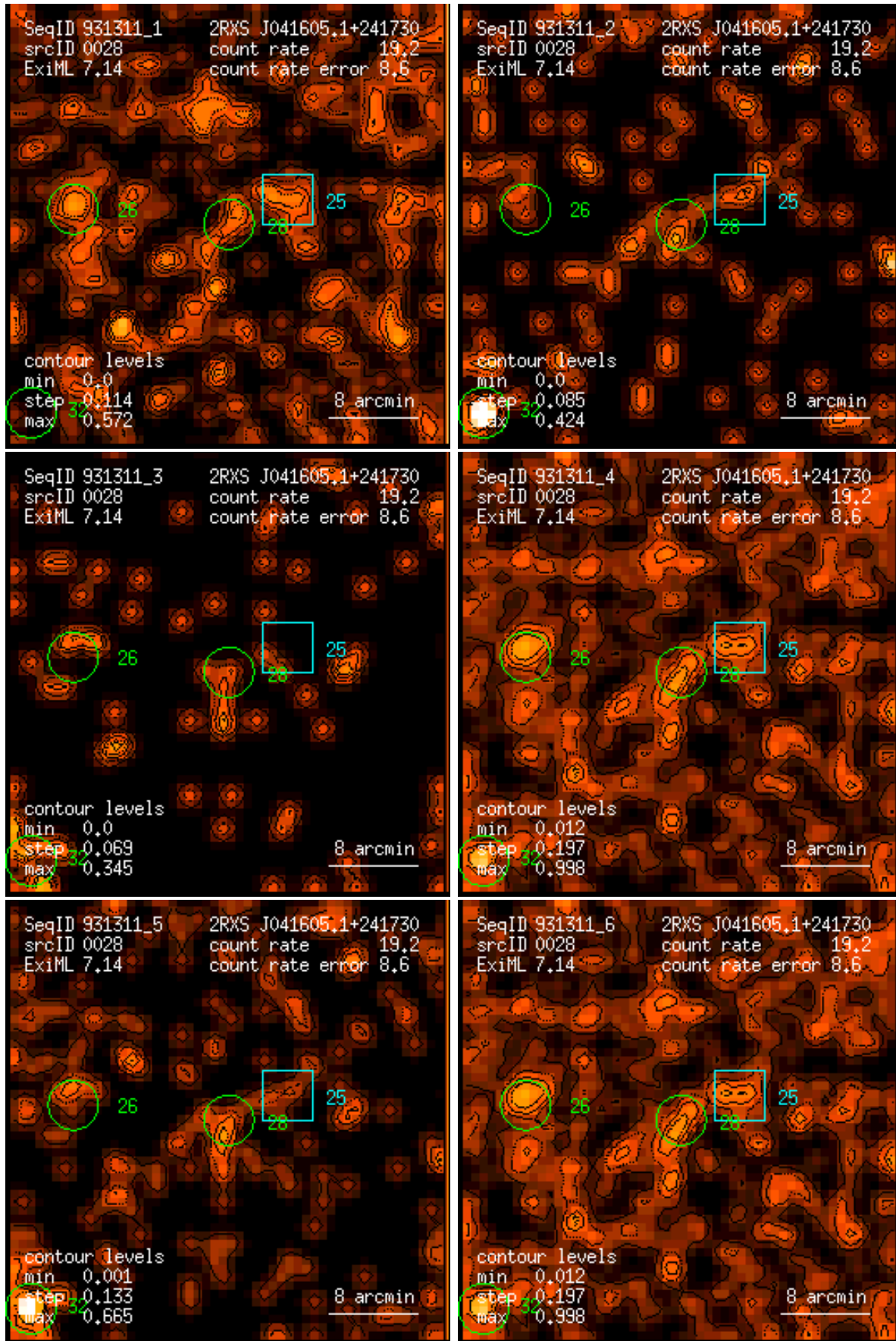
Figure 28: RASS 931311: detection 0028: band rate images, Gaussian filter: (1) PSPC channels 11 – 41, (2) 52 – 90, (3) 91 – 201, (4) 11 – 235, (5) 52 – 201, (6) 11 – 201. Broad band rates in counts/ks. Band rate contour levels in counts/ks/arcmin 2 .
