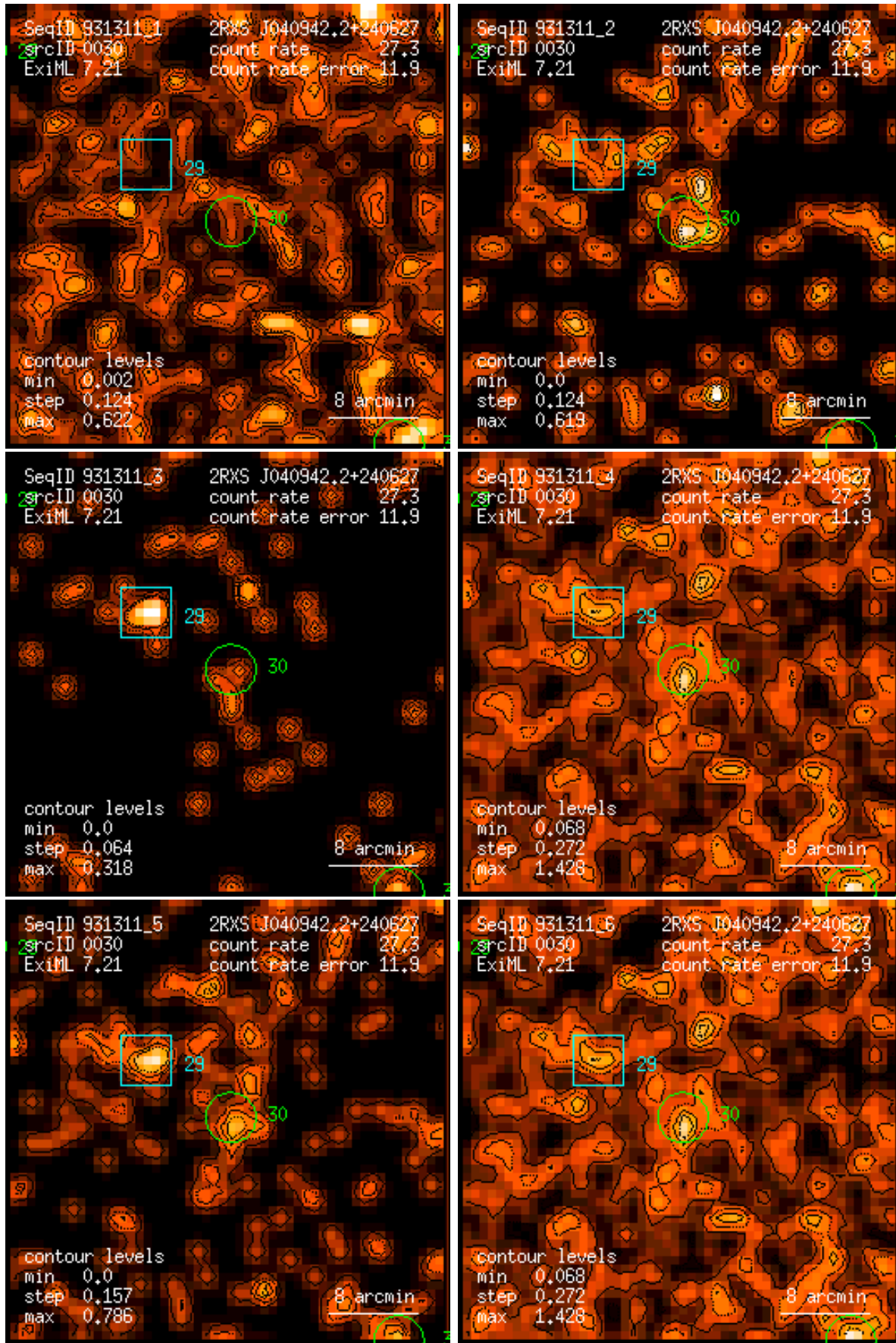
Figure 30: RASS 931311: detection 0030: band rate images, Gaussian filter: (1) PSPC channels 11 – 41, (2) 52 – 90, (3) 91 – 201, (4) 11 – 235, (5) 52 – 201, (6) 11 – 201. Broad band rates in counts/ks. Band rate contour levels in counts/ks/arcmin 2 .
