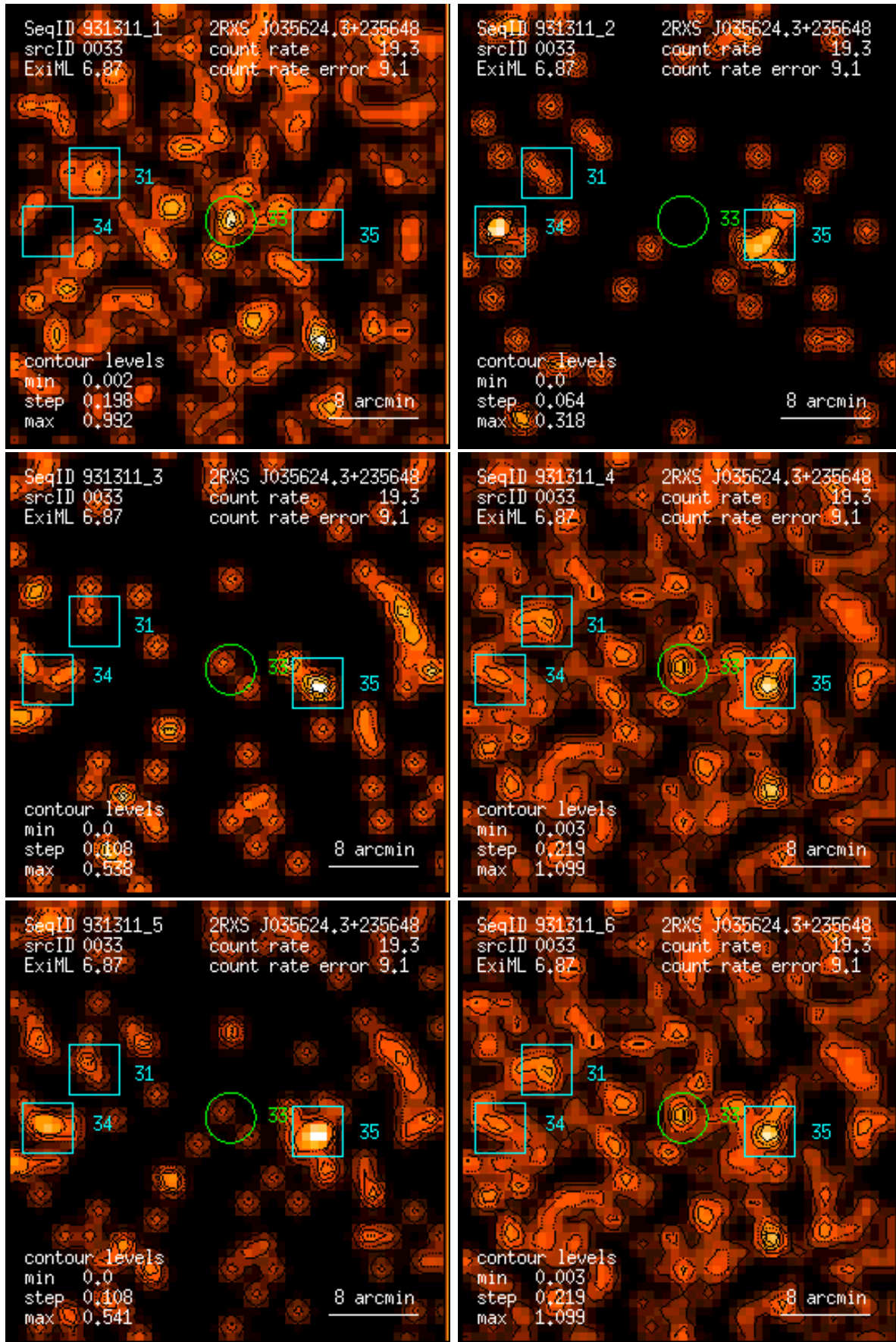
Figure 33: RASS 931311: detection 0033: band rate images, Gaussian filter: (1) PSPC channels 11 – 41, (2) 52 – 90, (3) 91 – 201, (4) 11 – 235, (5) 52 – 201, (6) 11 – 201. Broad band rates in counts/ks. Band rate contour levels in counts/ks/arcmin 2 .
