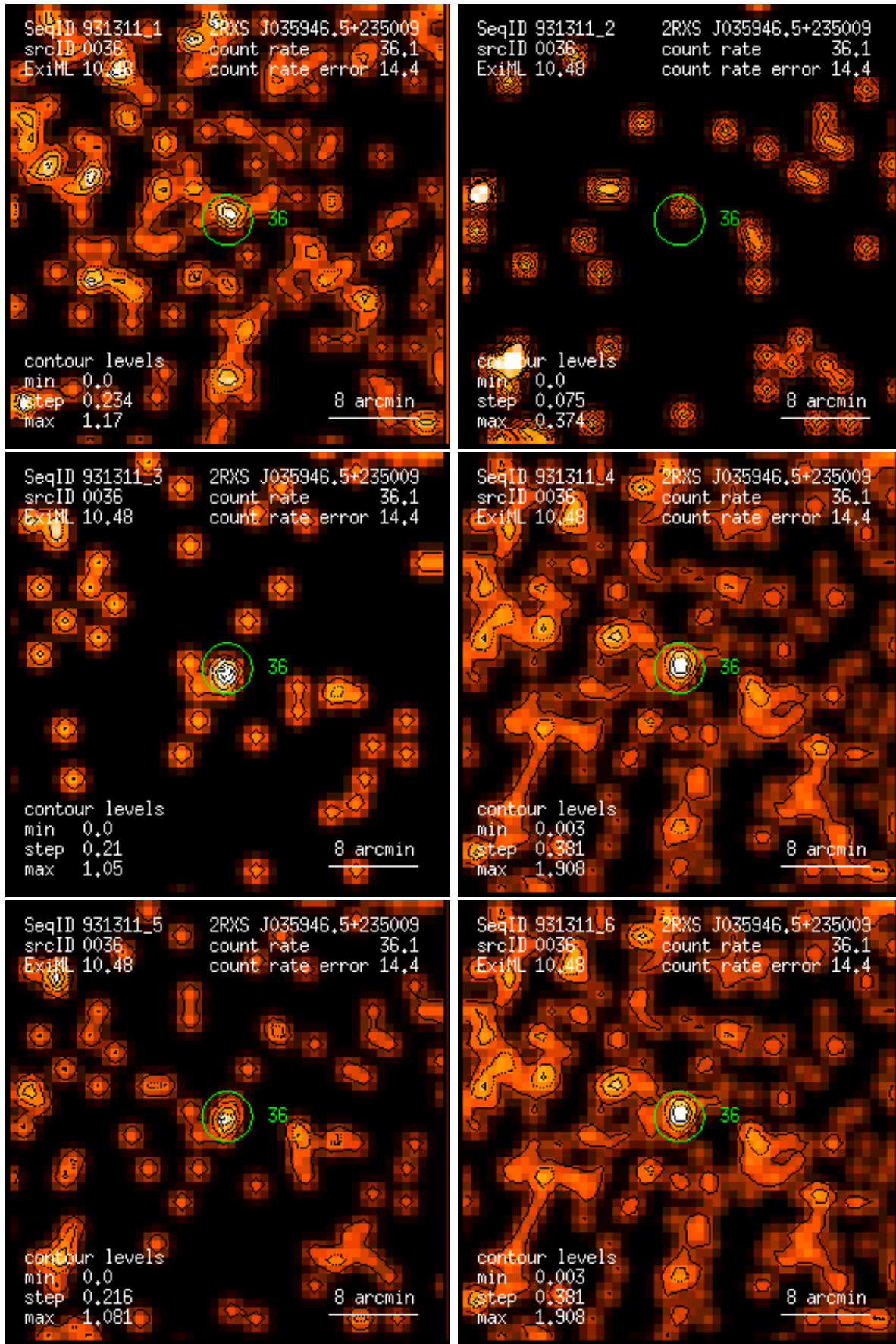
Figure 36: RASS 931311: detection 0036: band rate images, Gaussian filter: (1) PSPC channels 11 – 41, (2) 52 – 90, (3) 91 – 201, (4) 11 – 235, (5) 52 – 201, (6) 11 – 201. Broad band rates in counts/ks. Band rate contour levels in counts/ks/arcmin 2 .
