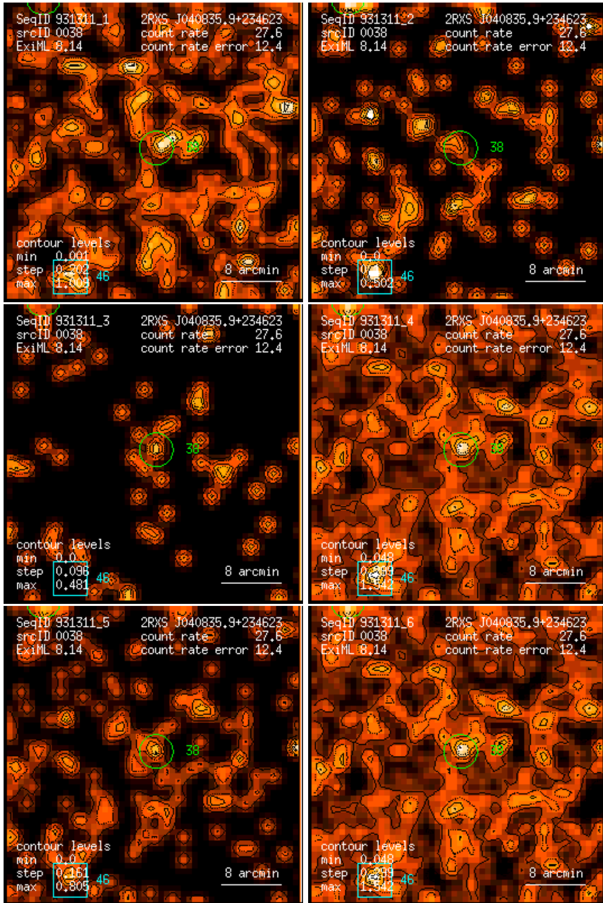
Figure 38: RASS 931311: detection 0038: band rate images, Gaussian filter: (1) PSPC channels 11 – 41, (2) 52 – 90, (3) 91 – 201, (4) 11 – 235, (5) 52 – 201, (6) 11 – 201. Broad band rates in counts/ks. Band rate contour levels in counts/ks/arcmin 2 .
